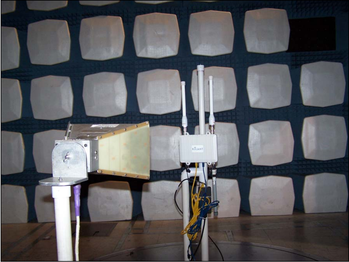
Photograph 4. Test Setup
