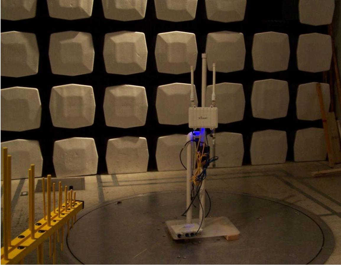
Photograph 2. RE Test Setup AC-POE
