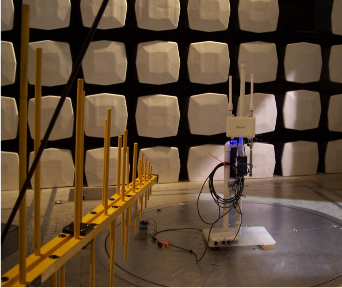
Photograph 3. RE Test Setup for DC-DC POE
