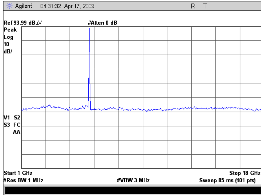
Plot 13. 802.11a Low Channel (chn 149), 1-18GHz
