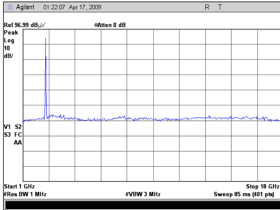
Plot 9. 2.4GHz High Channel, 1-18GHz (b mode)
