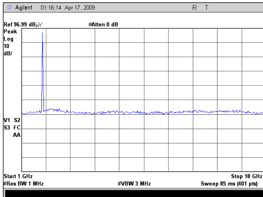
Plot 8. 2.4GHz Mid Channel, 1-18GHz (b mode)
