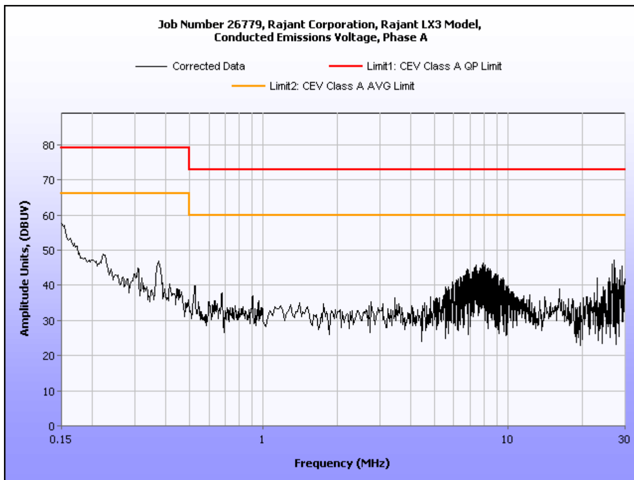
Plot 5. Conducted Emission, Phase Line Plot, (Model LX3-2250)
