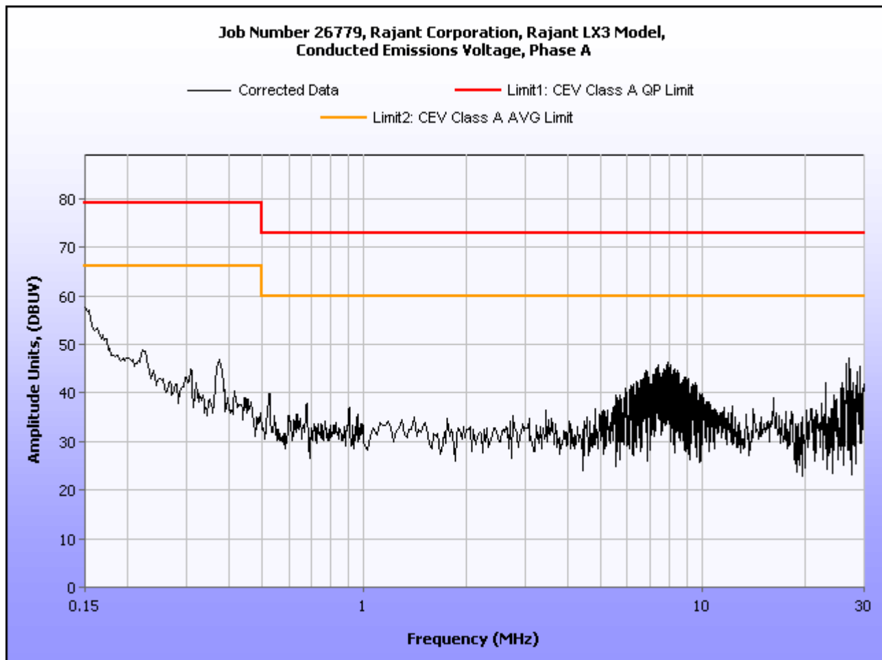
Plot 1. Conducted Emission, Phase Line Plot, (Model LX3-2250)
