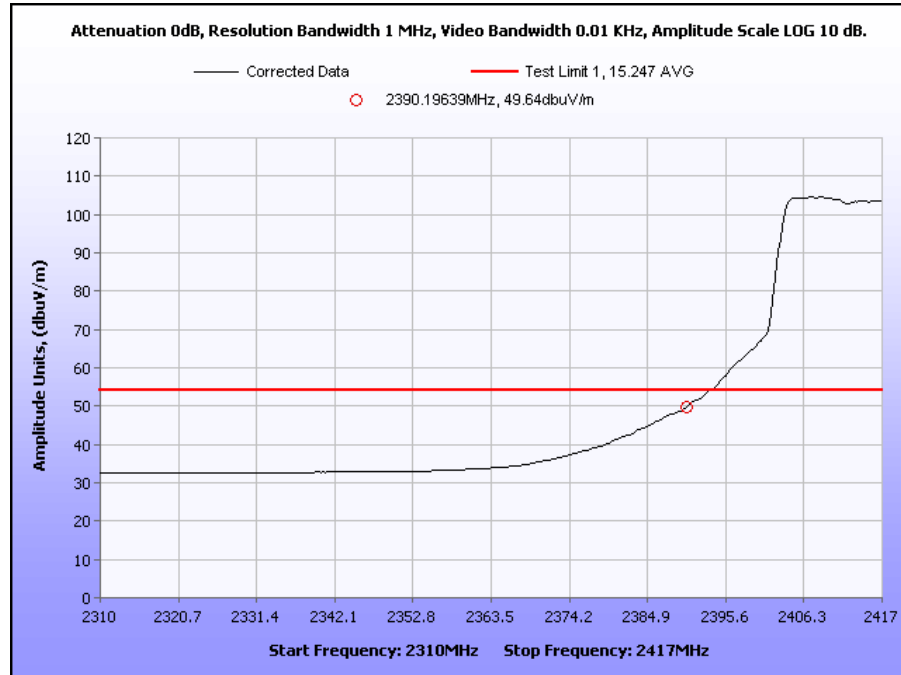
Plot 24. 2.4GHz Channel 1 Band Edge – Avg (g mode)
