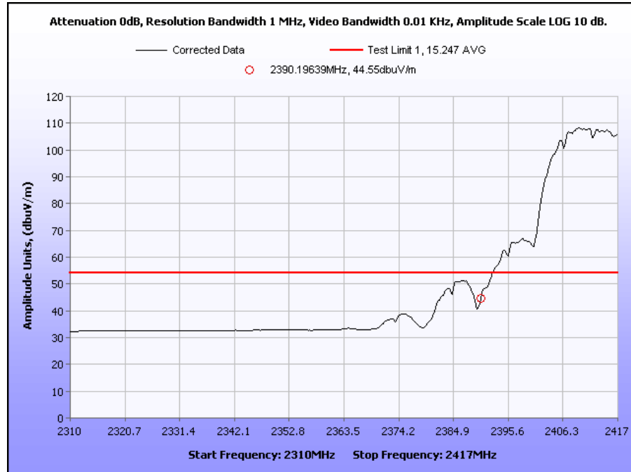
Plot 18. 2.4GHz Channel 1 Band Edge – Avg (b mode)
