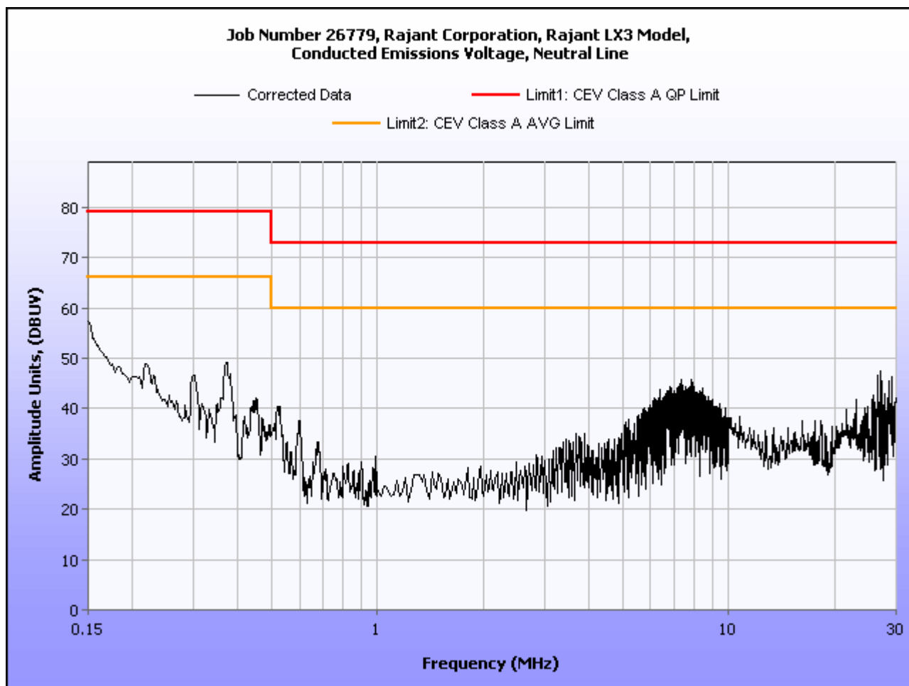
Plot 2. Conducted Emission, Neutral Line Plot, (Model LX3-2250)
