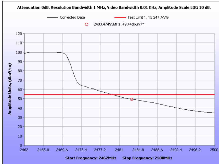
Plot 28. 2.4GHz Channel 11 Band Edge – Avg (g mode)
