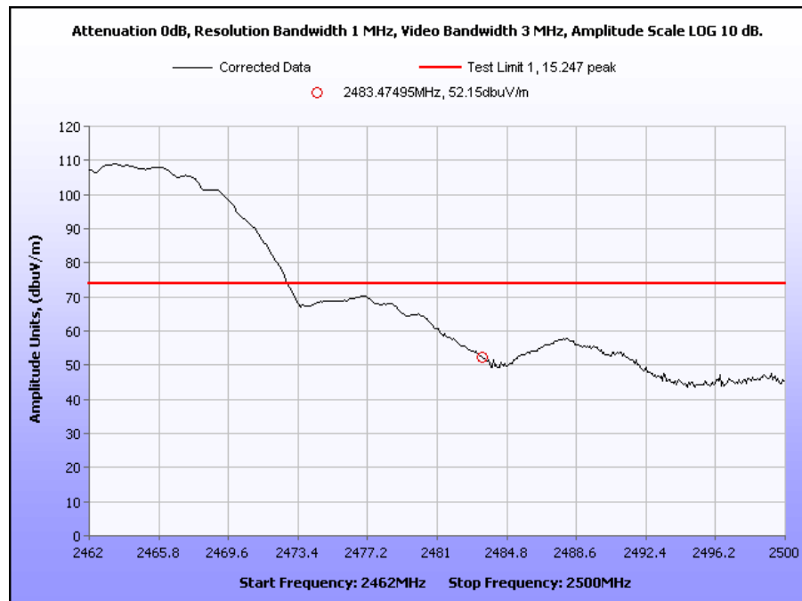
Plot 23. 2.4GHz Channel 11 Band Edge – Peak (b mode)
