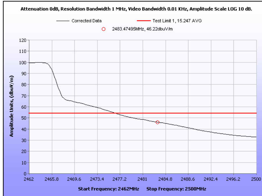
Plot 26. 2.4GHz Channel 10 Band Edge – Avg (g mode)
