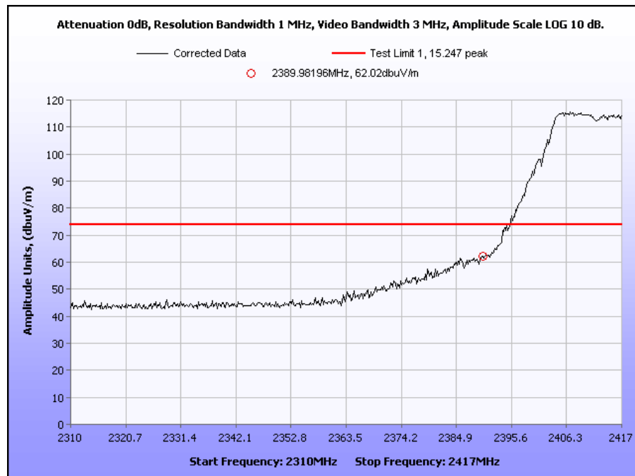
Plot 25. 2.4GHz Channel 1 Band Edge – Peak (g mode)
