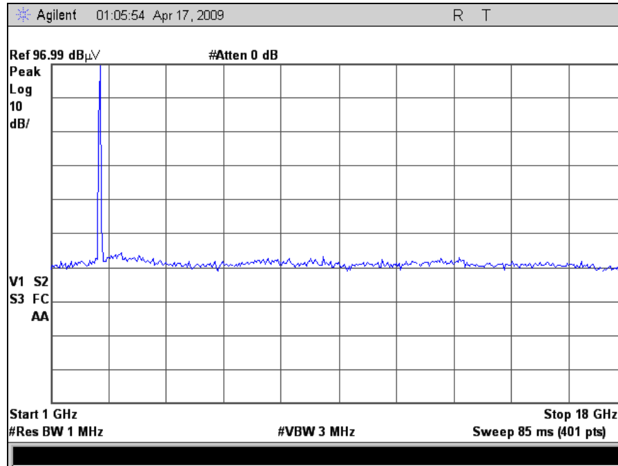
Plot 10. 2.4GHz Low Channel, 1-18GHz (g mode)
