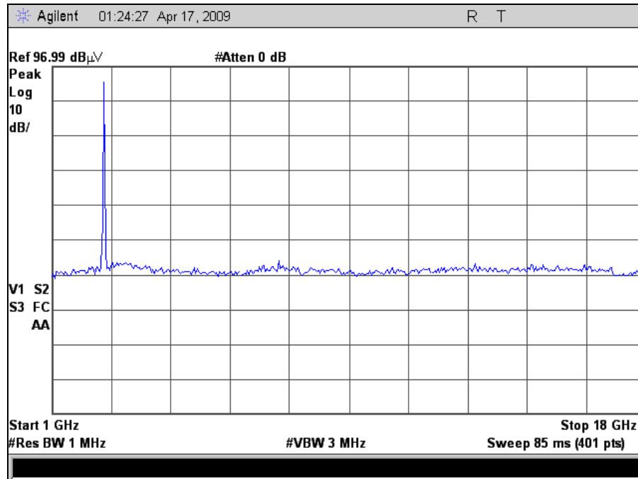
Plot 12. 2.4GHz High Channel, 1-18GHz (g mode)
