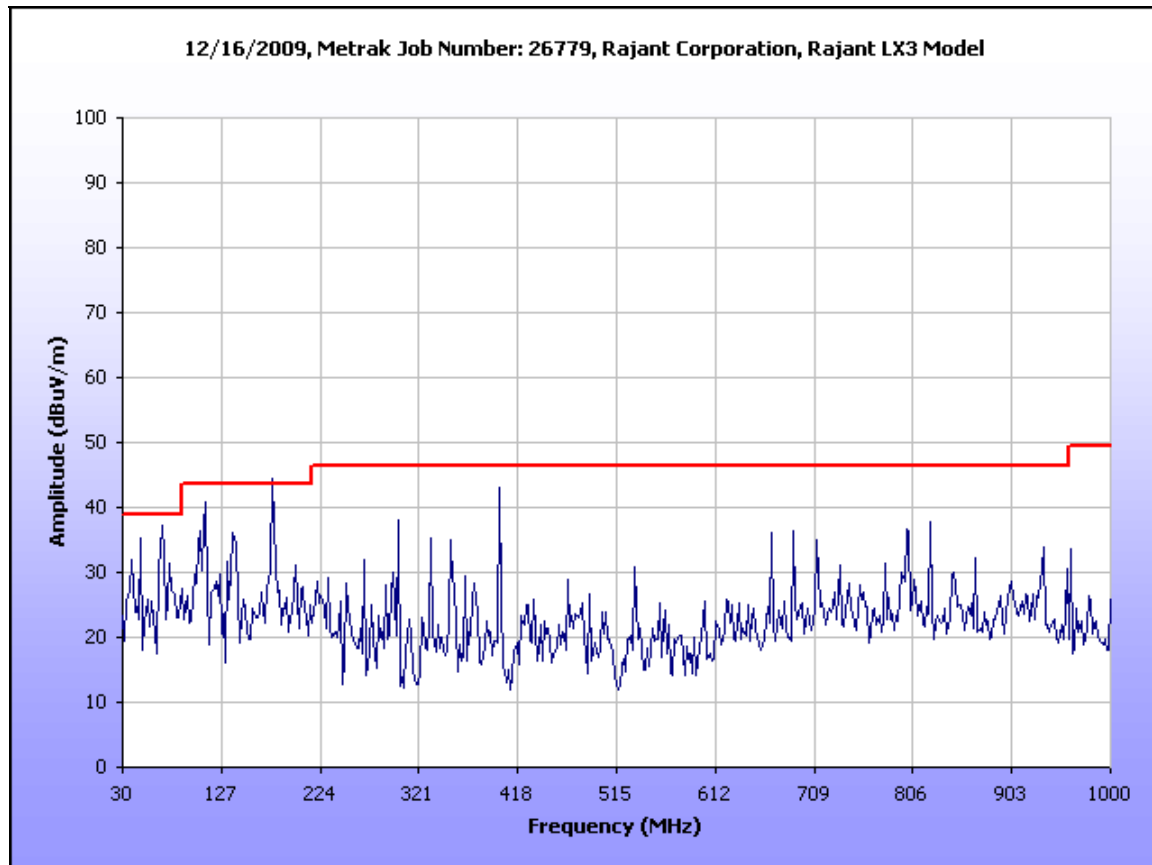
Plot 4. Radiated Emissions Limits Test Results, 30 MHz – 1 GHz, Model LX3-2250 (AC POE)
