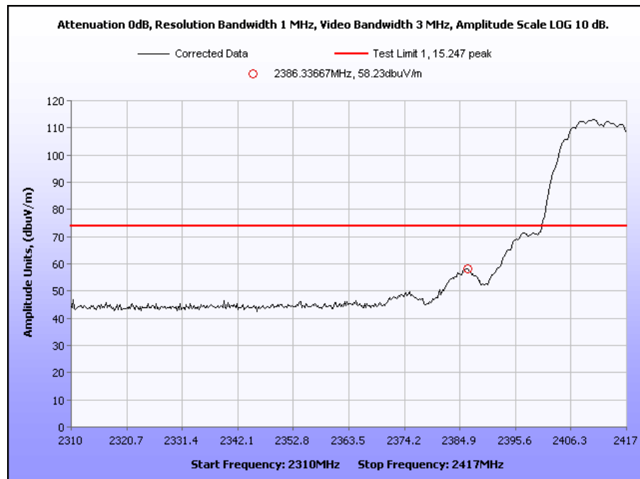
Plot 19. 2.4GHz Channel 1 Band Edge – Peak (b mode)
