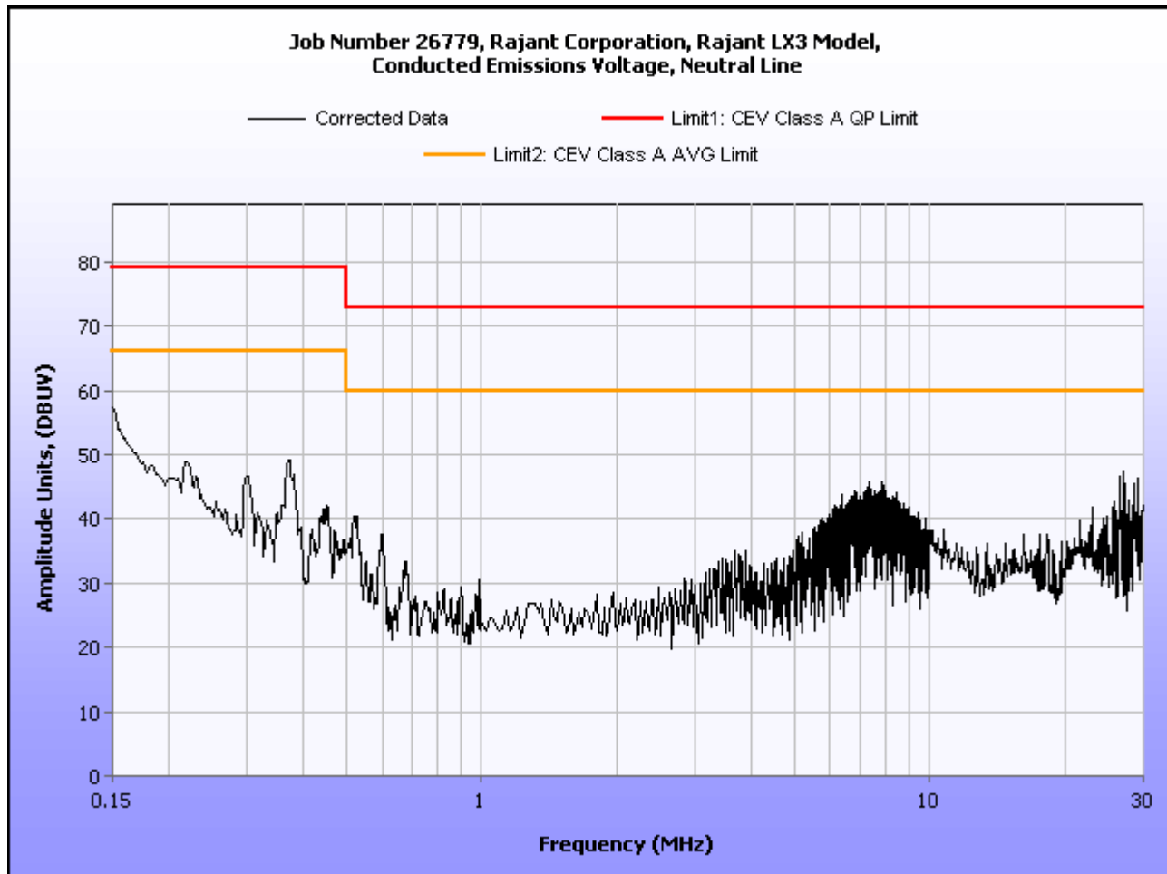
Plot 6. Conducted Emission, Neutral Line Plot, (Model LX3-2250)
