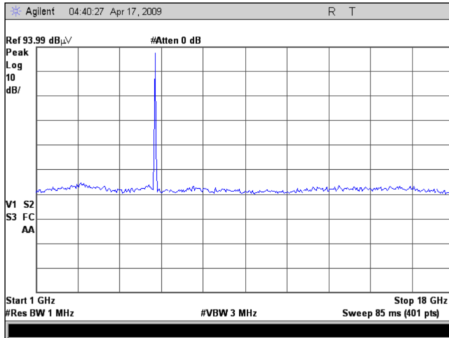
Plot 15. 802.11a High Channel (chn 165), 1-18GHz
