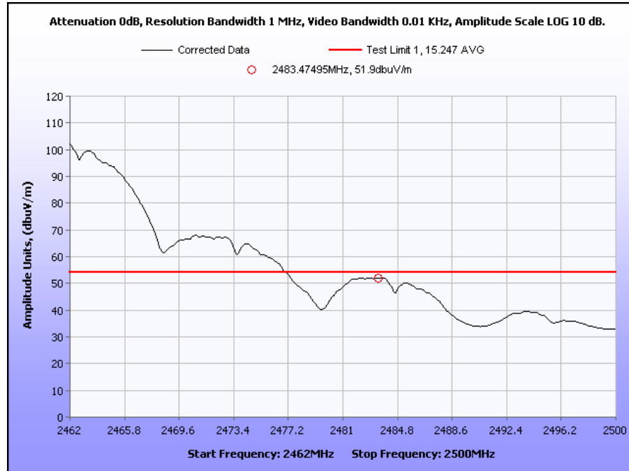
Plot 20. 2.4GHz Channel 10 Band Edge – Avg (b mode)
