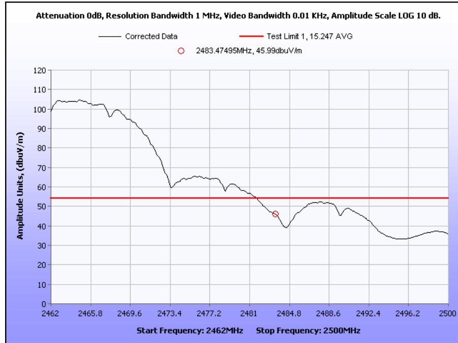
Plot 22. 2.4GHz Channel 11 Band Edge – Avg (b mode)
