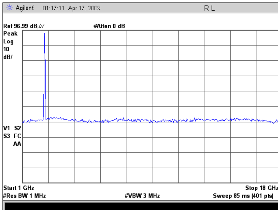
Plot 11. 2.4GHz Mid Channel, 1-18GHz (g mode)
