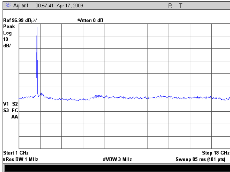
Plot 7. 2.4GHz Low Channel, 1-18GHz (b mode)
