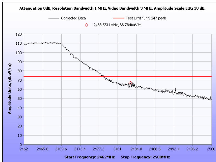
Plot 29. 2.4GHz Channel 11 Band Edge – Peak (g mode)
