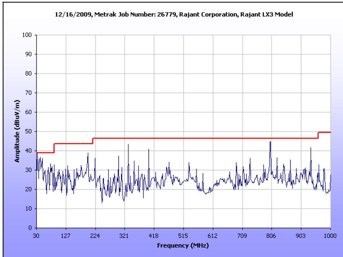
Plot 3. Radiated Emissions Limits Test Results, 30 MHz – 1 GHz, Model LX3-2250 (DC POE)
