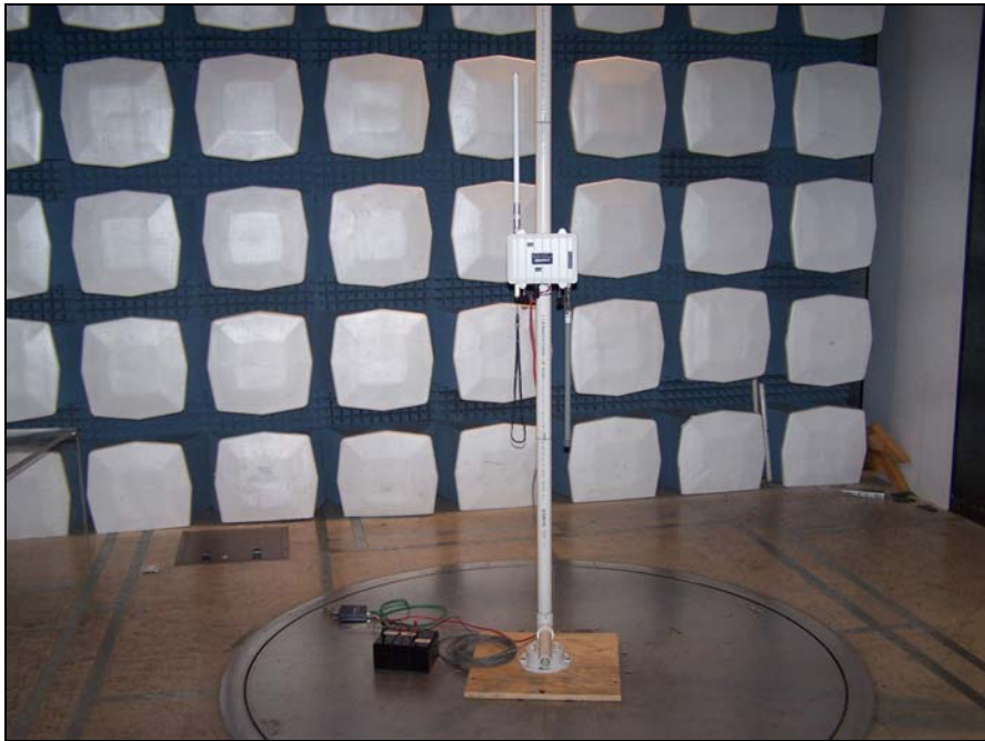
Photograph 6. Radiated Emissions
