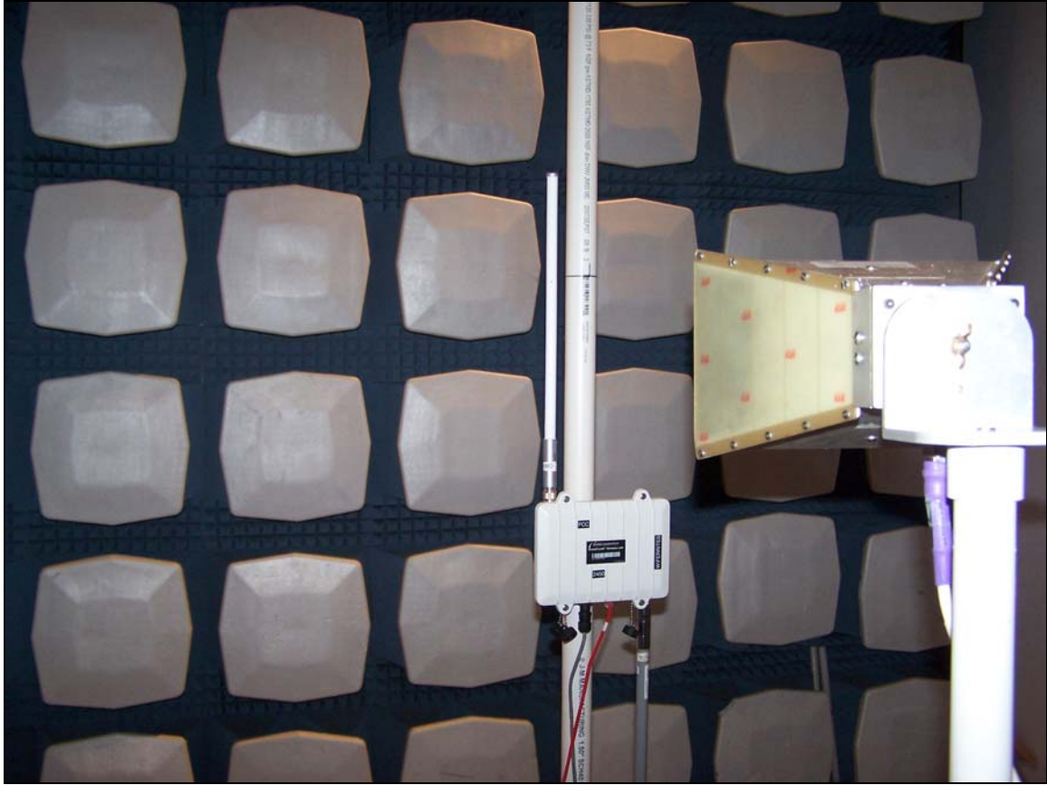
Photograph 1. Radiated Setup, 5.8 Mode
