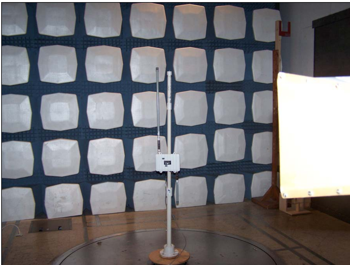
Photograph 4. Harmonics Setup, 900 MHz
