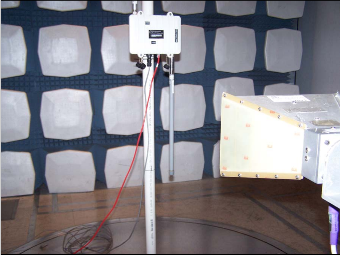
Photograph 2. Radiated Setup, b and g Modes
