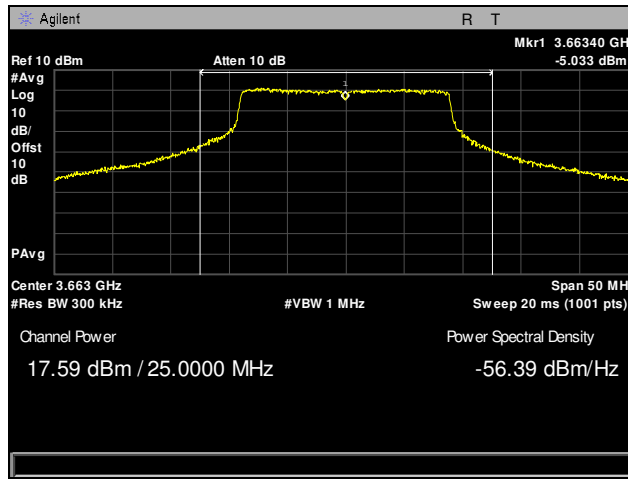
Plot 7. Measured Power, Low Channel, BW 20 MHz, Chain 0, 2 dBi Antenna
