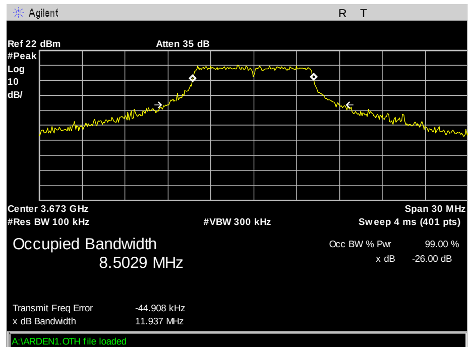
Plot 70. Occupied Bandwidth - Mid - 3673.4MHz - BW10MHz - Chain1
