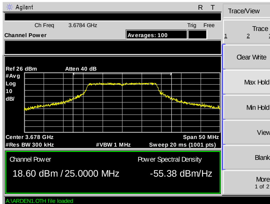
Plot 3. Measured Power - Mid - 3678.4MHz - BW20MHz - Chain0 - 2dBi Antenna
