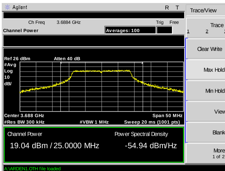
Plot 5. Measured Power - High - 3688.4MHz - BW20MHz - Chain0 - 2dBi Antenna
