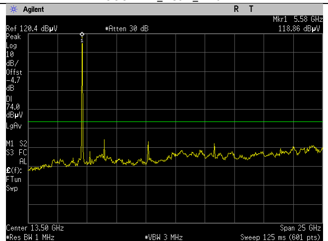
5600MHz_Ch_120_20MHz BW_a-mode_1-26GHz _Peak_Ant D
