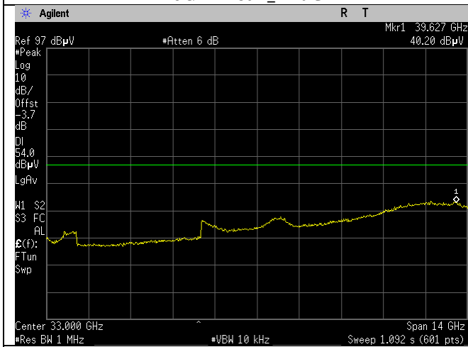
5320MHz_High Ch_64_20MHz BW_a-mode_26- 40GHz_Avg_Ant C
