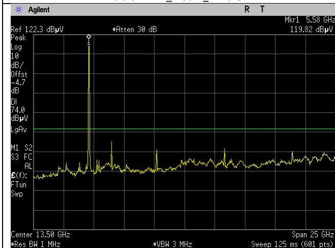
5600MHz_Ch_120_20MHz BW_a-mode_1-26GHz _Peak_Ant C
