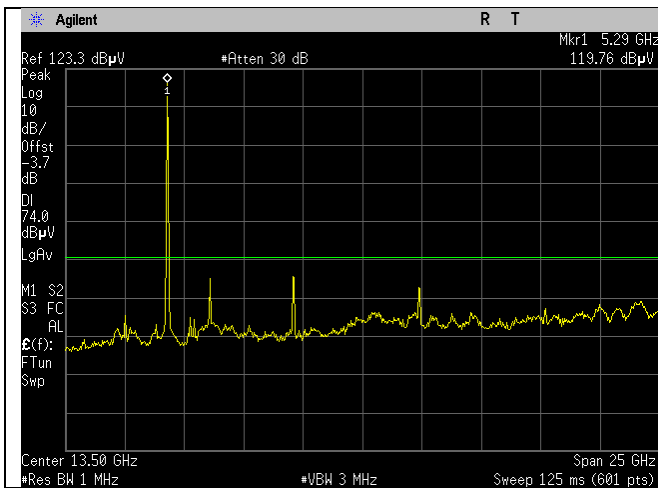
5300MHz_high_Mid Ch_60_20MHz BW_a-mode_1-26GHz_Peak_Ant C
