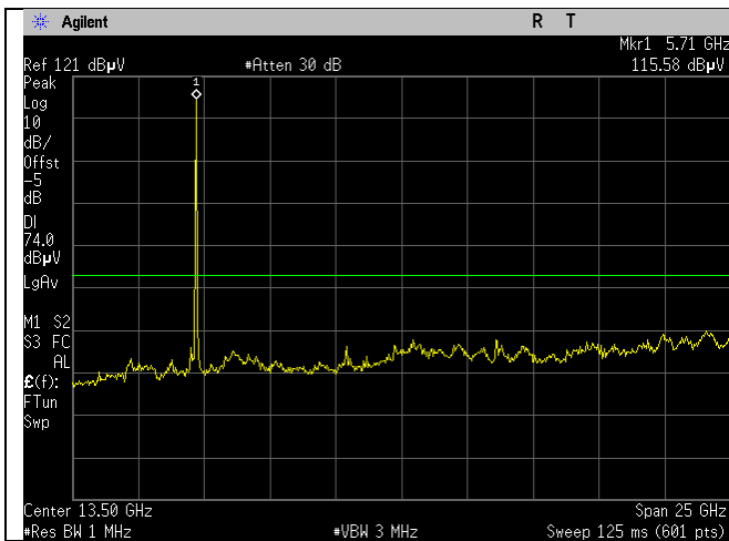
5700MHz_Ch_140_20MHz BW_a-mode_1-26GHz _Peak_Ant A
