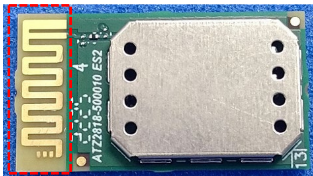
Figure 1: Antenna Appearance/アンテナ外観
