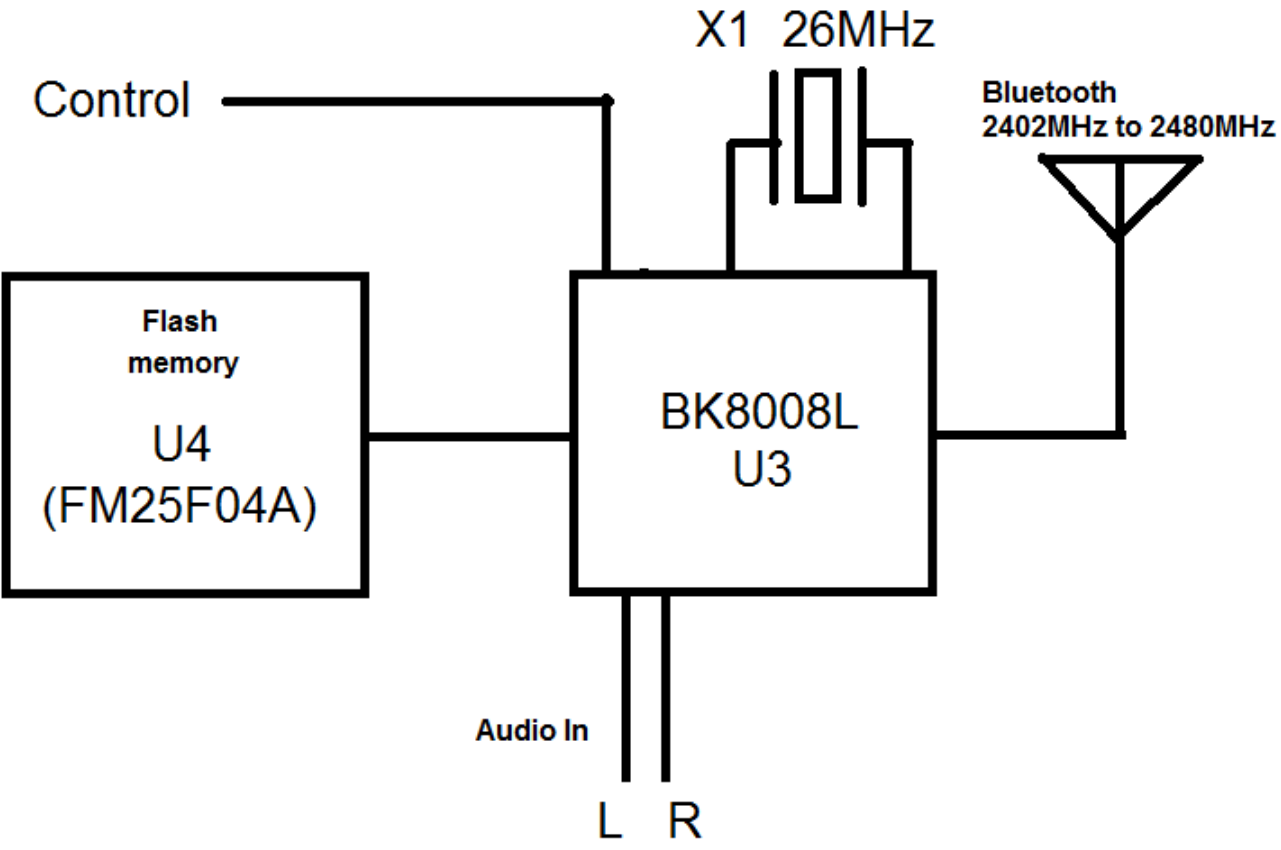
F-6008A Bluetooth Module Block Diagram
