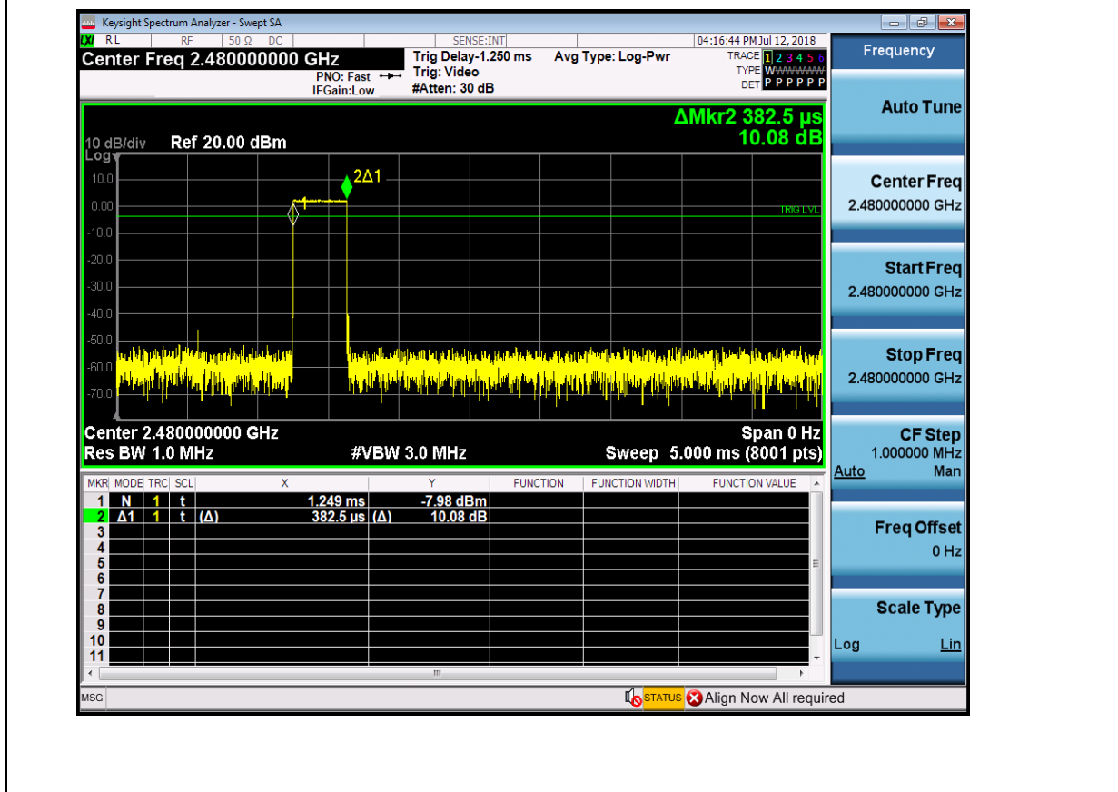
Dwell Time_DH1_2480
