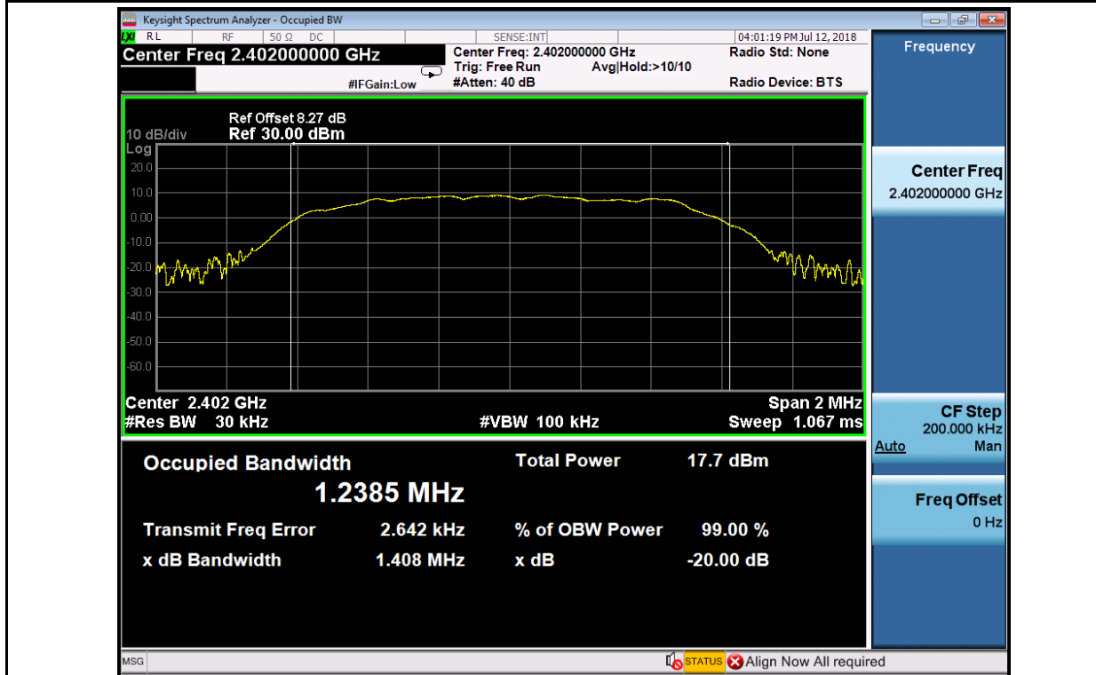
20 dB Bandwidth_3DH5_2402
