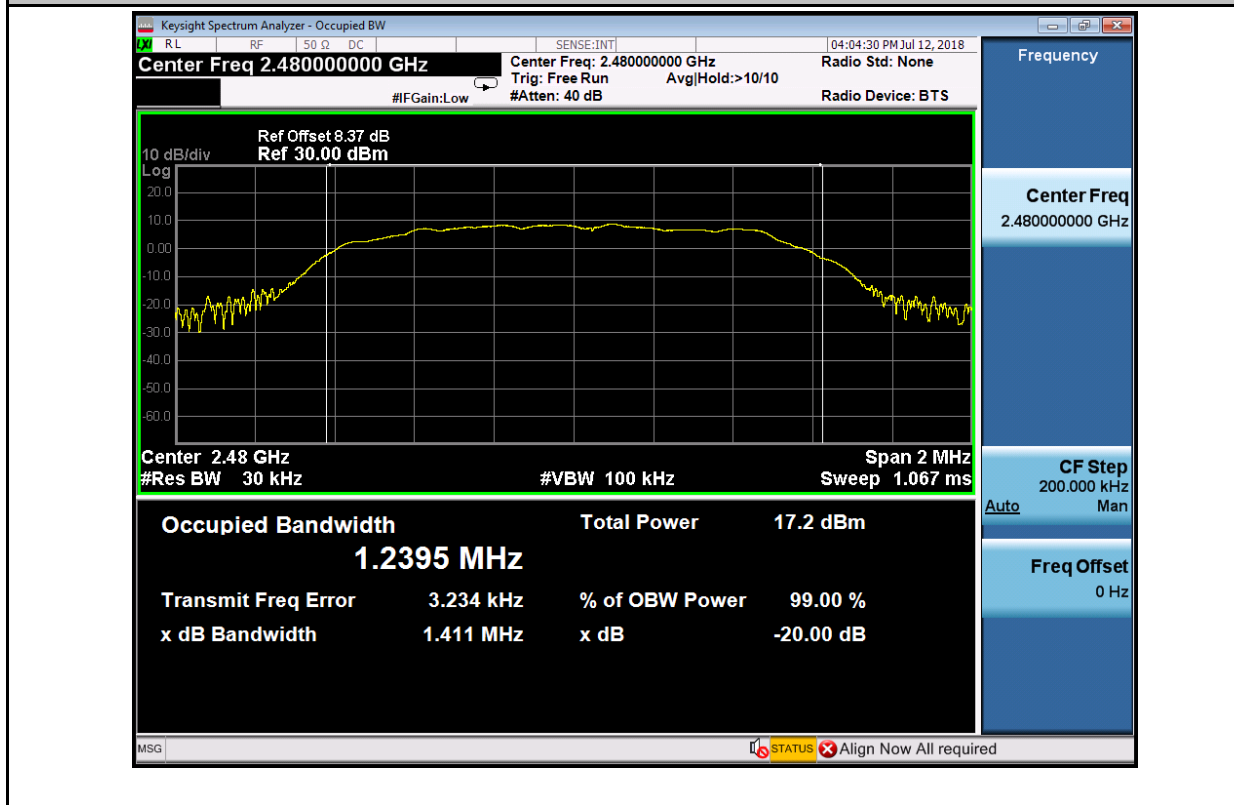
20 dB Bandwidth_3DH5_2480
