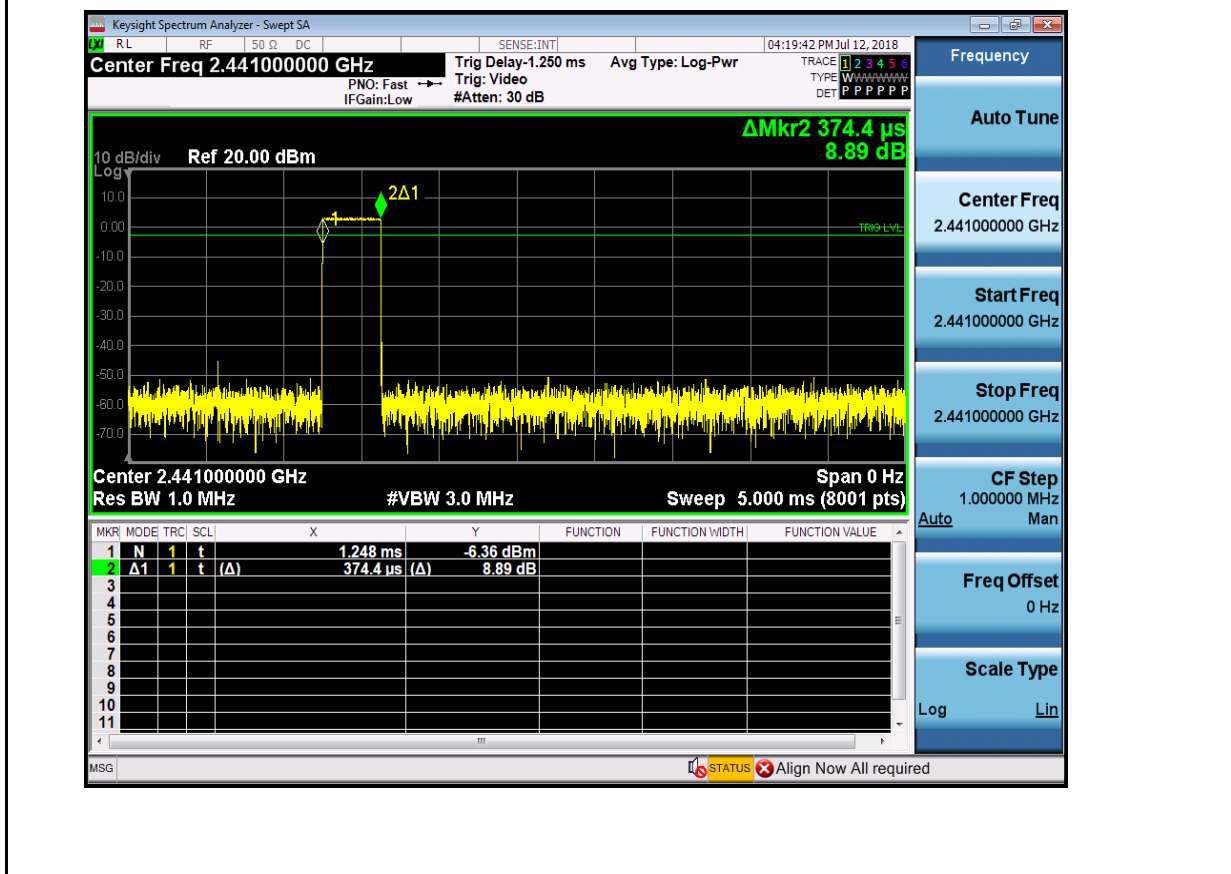
Dwell Time_DH1_2441
