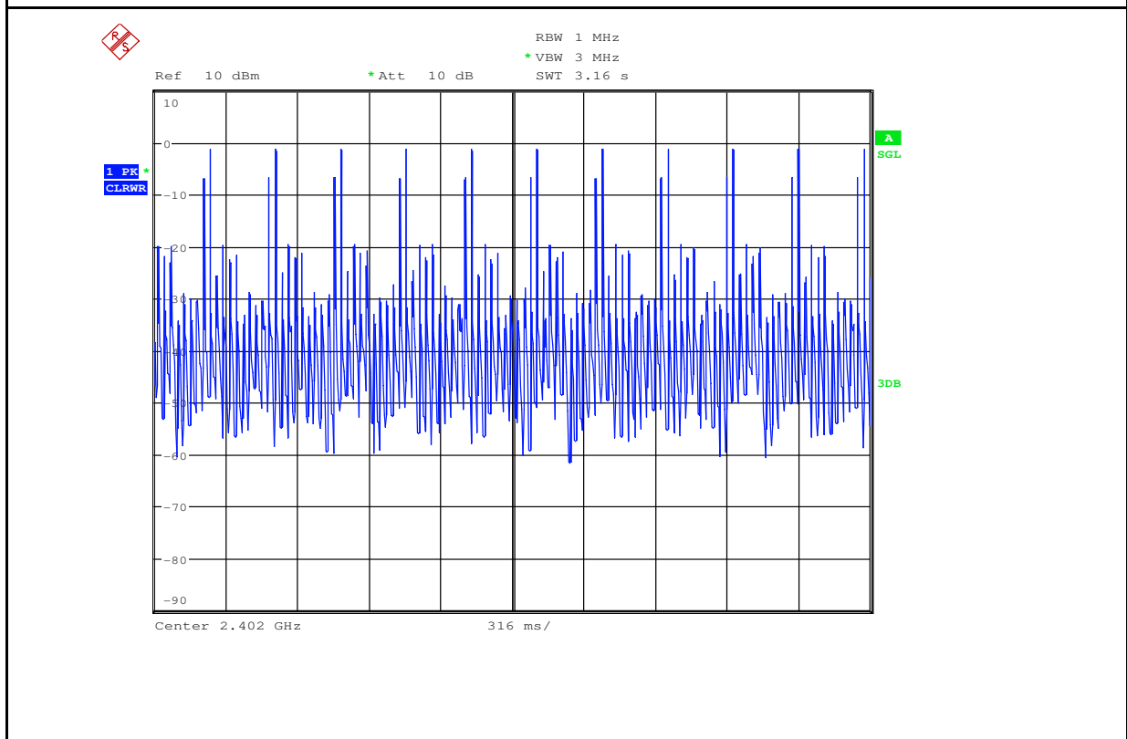
Dwell Time_3DH1_2402
