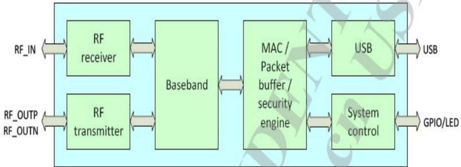
Figure 1 MT7601 block diagram
