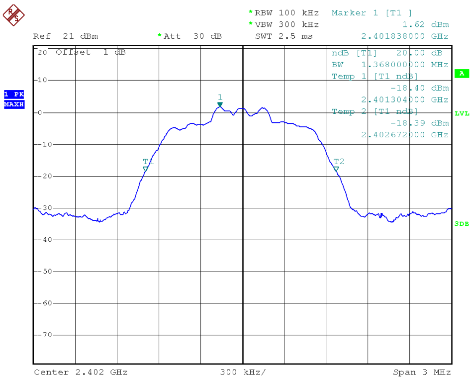
(Plot D: Channel = 2402 @ \pi/4 -DQPSK)
