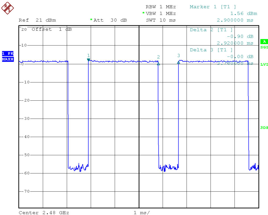
(Plot I: Channel = 2480 @ 8-DPSK)
