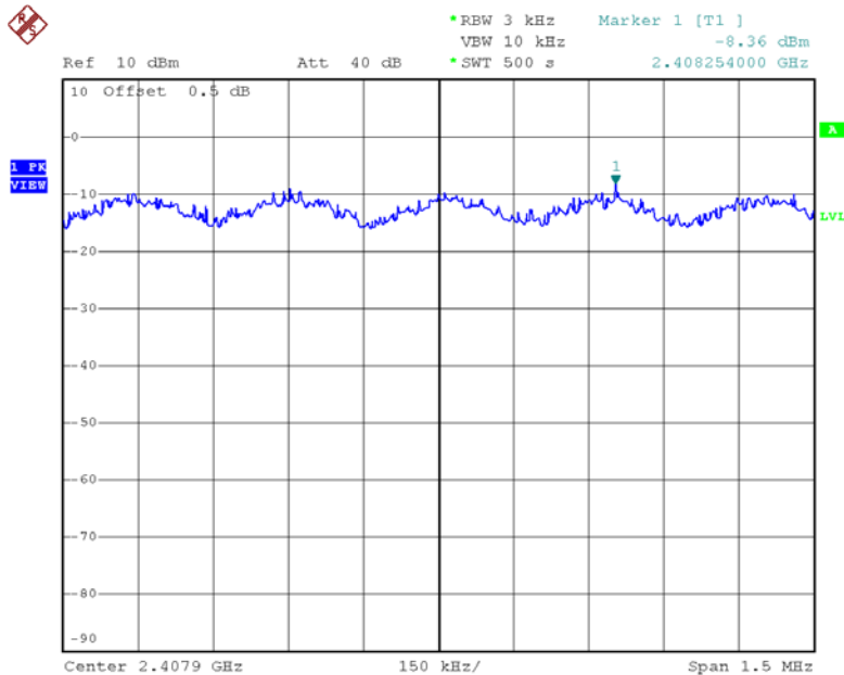
PLOT E6A : 802.11g, Lowest Channel, Antenna 1 (Con 2)
