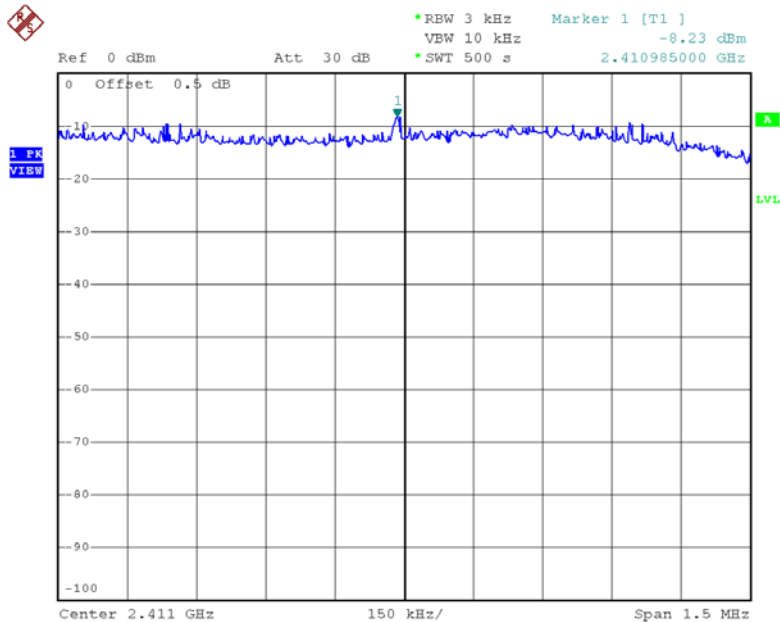
PLOT T5A : 802.11b, Lowest Channel, Antenna 0 (Con 1)
