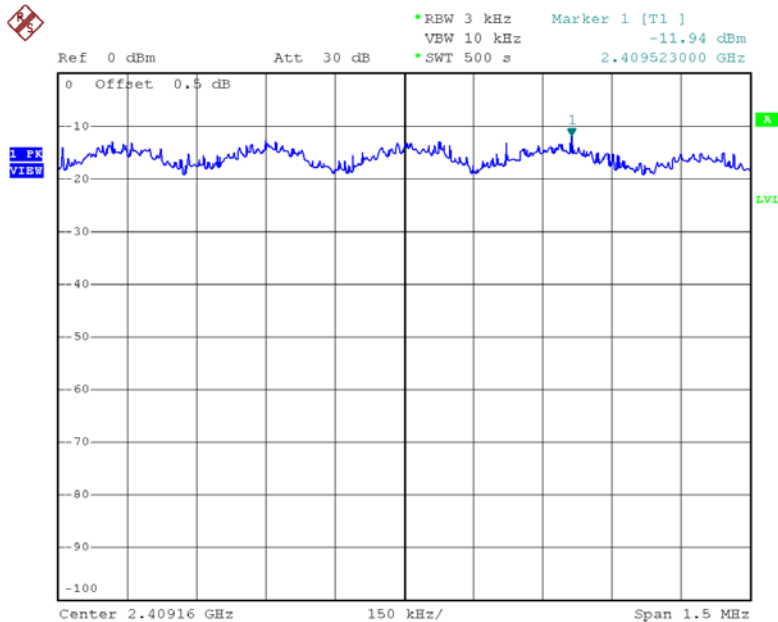
PLOT T6A : 802.11g, Lowest Channel, Antenna 0 (Con 1)
