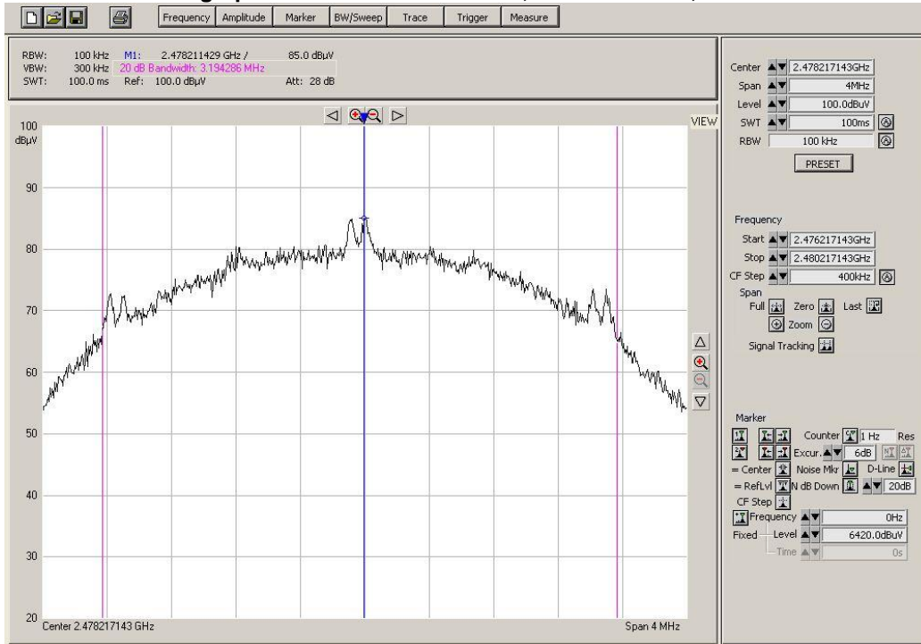
Figure 4 – Result data graph shows 20 dB bandwidth, CF = 2.478GHz, BW = 3.19MHz
