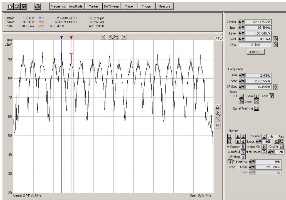
Figure 5 – Result data graph shows the channel separation:
