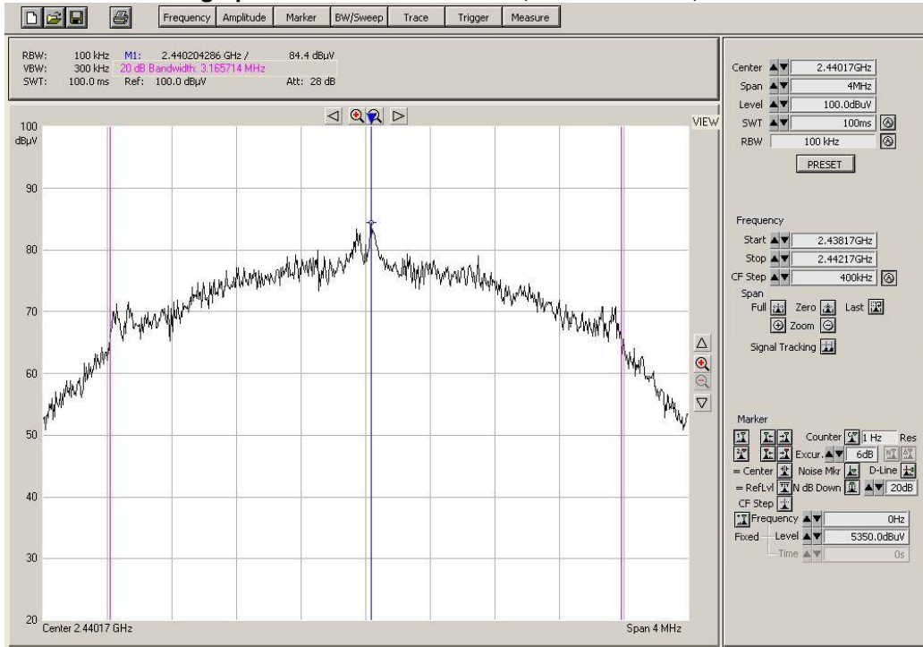
Figure 3 – Result data graph shows 20 dB bandwidth, CF = 2.440GHz, BW = 3.16MHz
