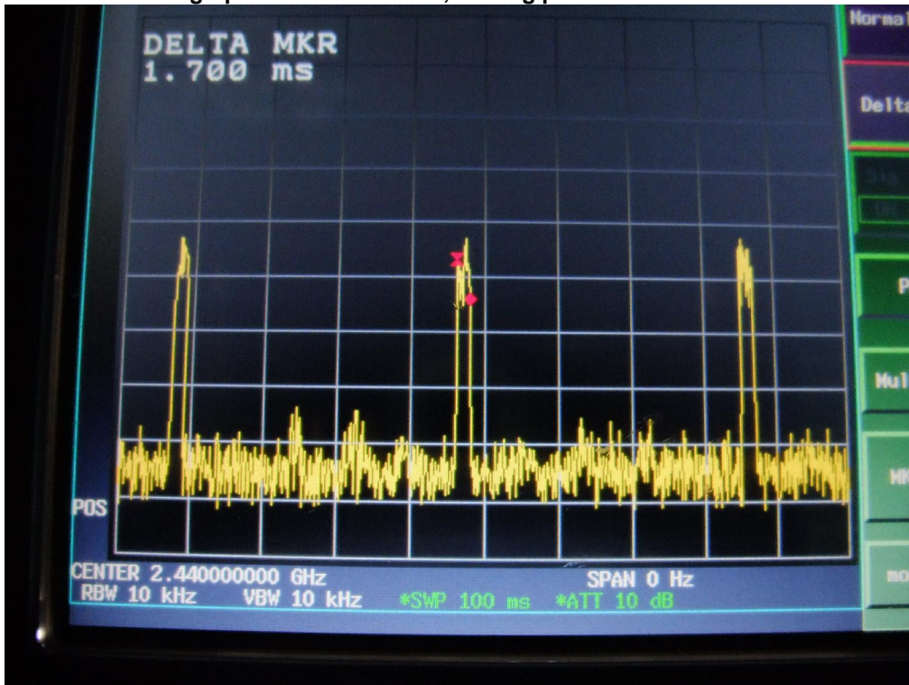
Figure 7 – Result data graph zooms into detail, one big pulse is built with 1.7ms.
