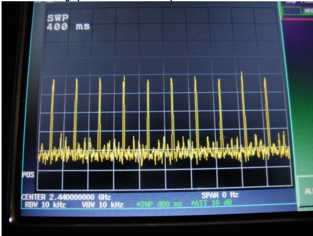
Figure 6 – Result data graph shows 400ms with 10 pulses.
