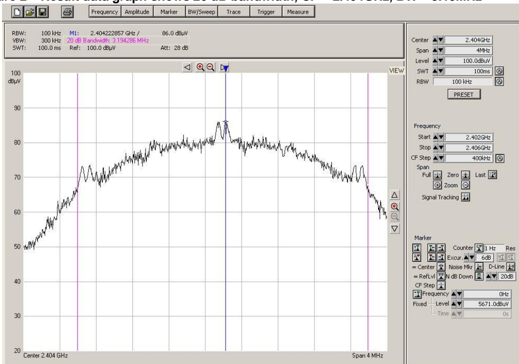
Figure 2 – Result data graph shows 20 dB bandwidth, CF = 2.404GHz, BW = 3.19MHz
