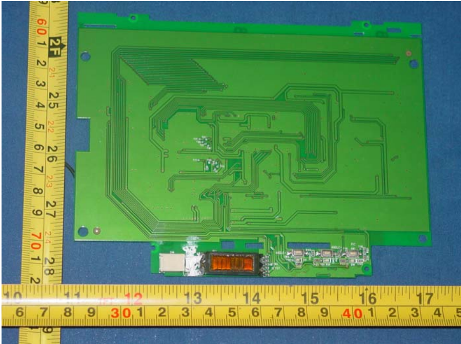
Figure 10 Internal photo of EUT
