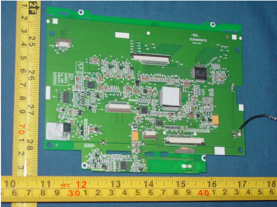
Figure 9 Internal photo of EUT
