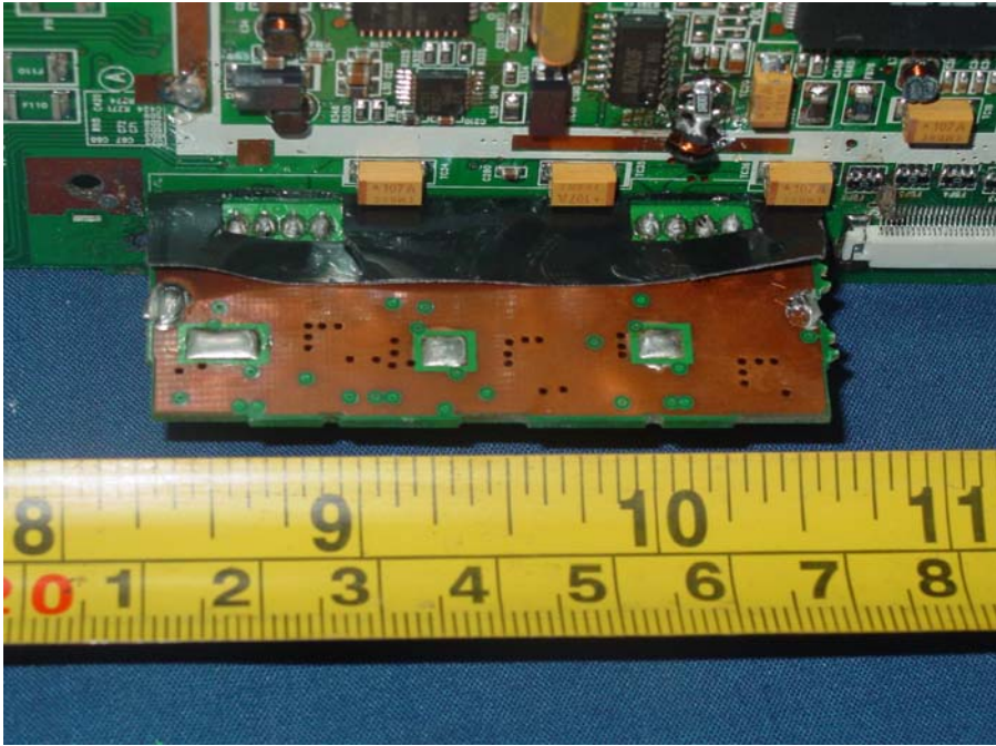
Figure 8 Internal photo of EUT
