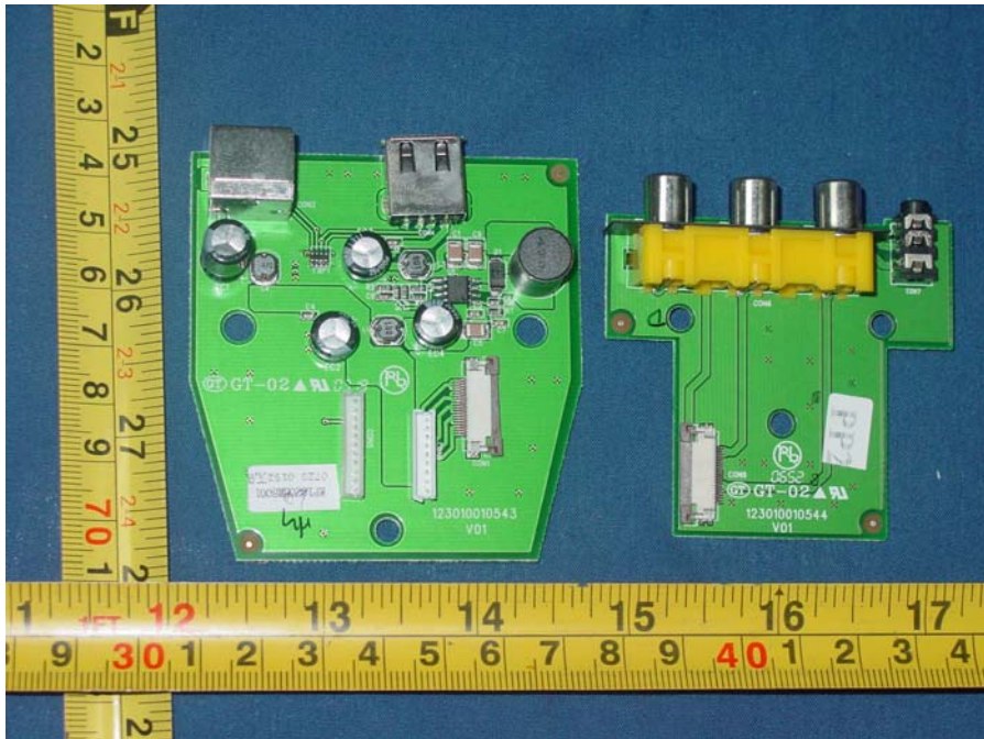
Figure 19 Internal photo of EUT
