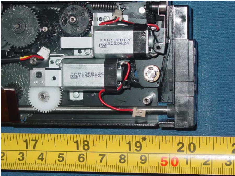
Figure 17 Internal photo of EUT
