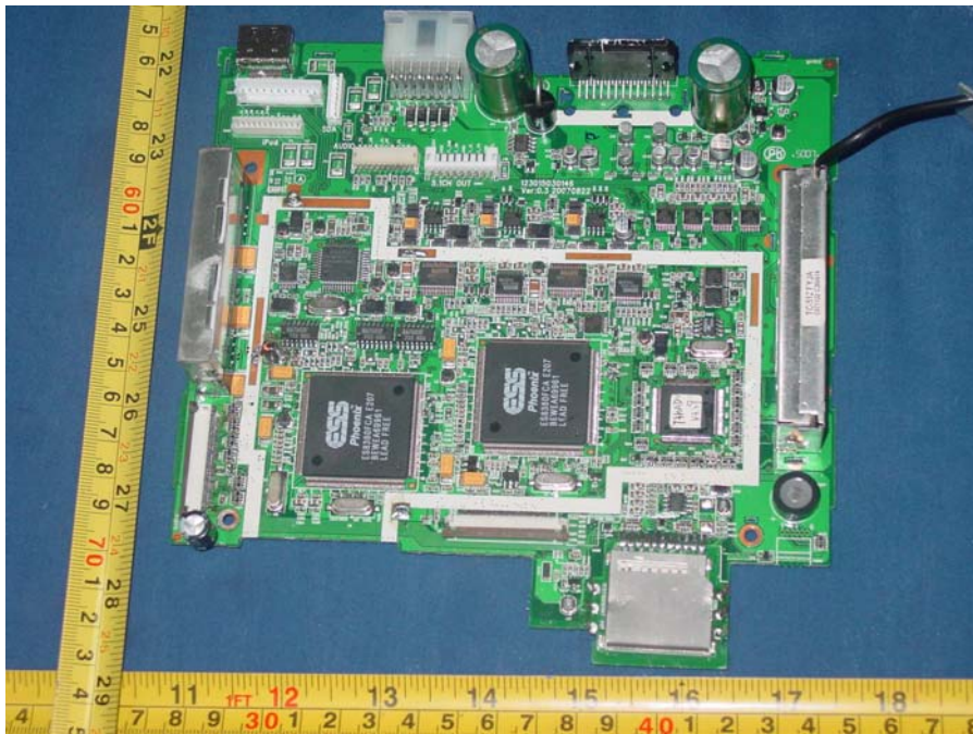
Figure 4 Internal photos 4 of EUT
