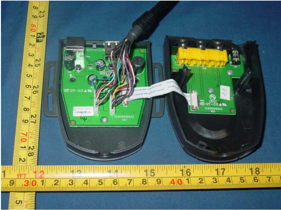
Figure 18 Internal photo of EUT
