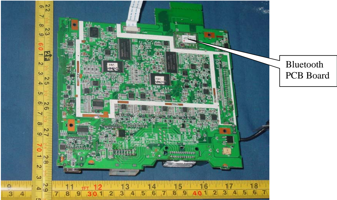
Figure 5 Internal photo of EUT
