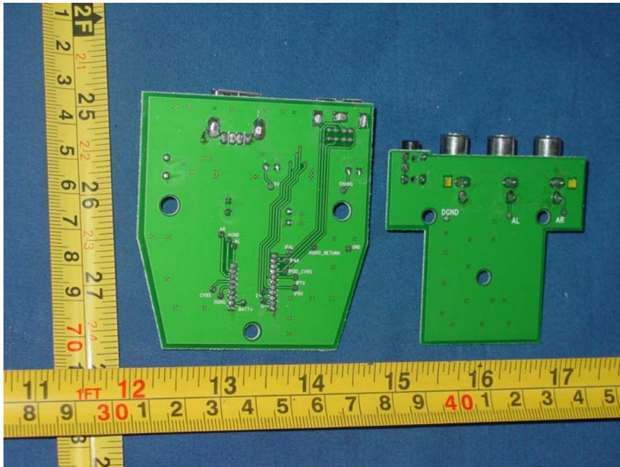
Figure 20 Internal photo of EUT
