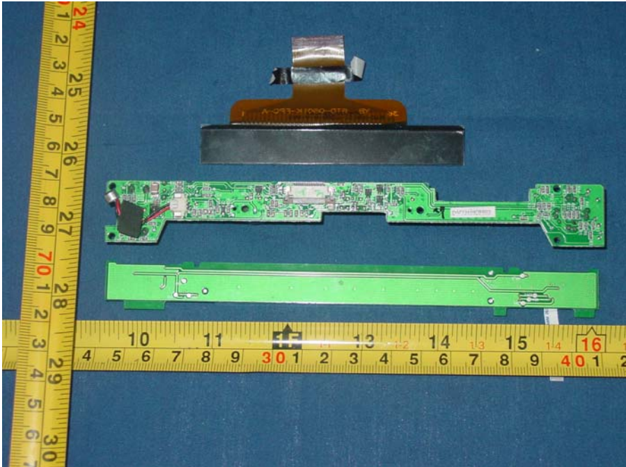
Figure 16 Internal photo of EUT
