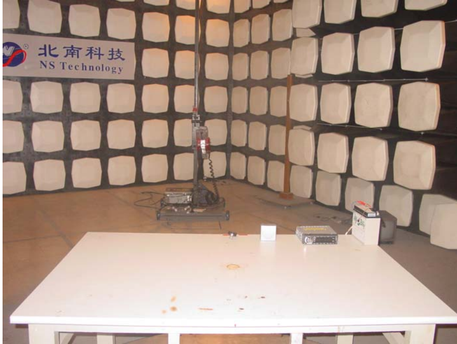
Figure 5 Test photo of Transmitter Spurious Emission (Normal operation 1000-18000MHz)
