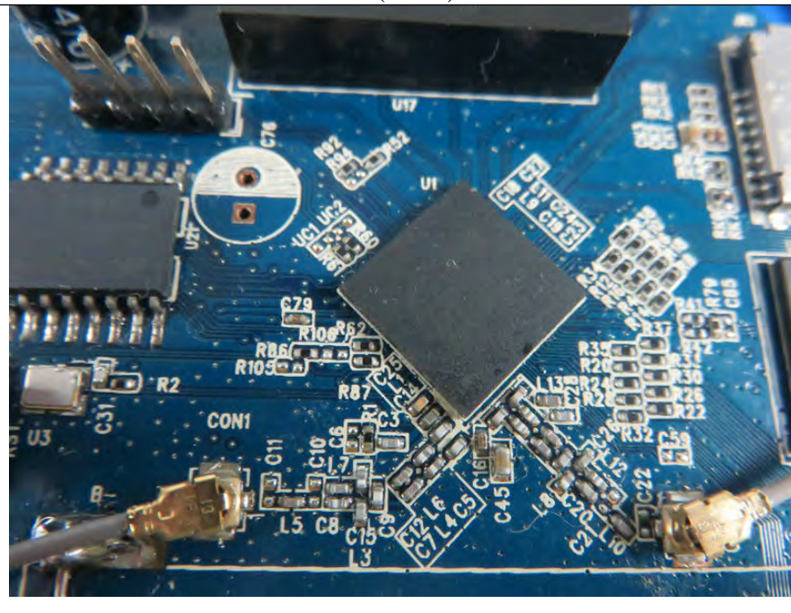
4. Figure PCB of the EUT-Module View (WIFI)
