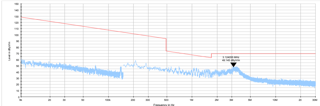
Plot 7.3.3 Radiated emission measurements from 9 kHz to 30 MHz at the high carrier frequency
