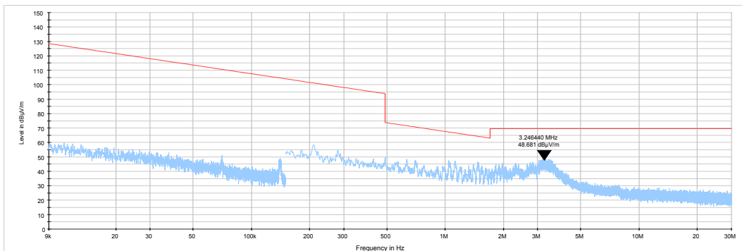
Plot 7.3.2 Radiated emission measurements from 9 kHz to 30 MHz at the mid carrier frequency
