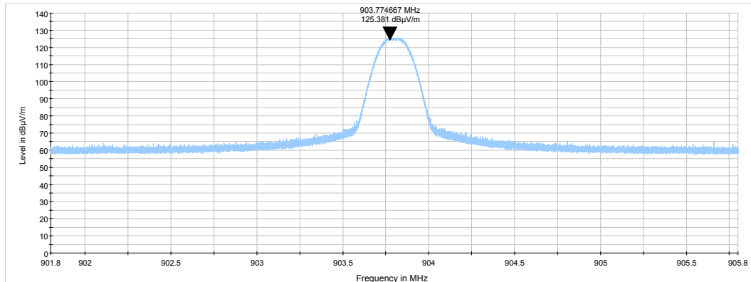
Plot 7.2.11 Field strength of carrier at mid frequency GFSK 50 kbps
