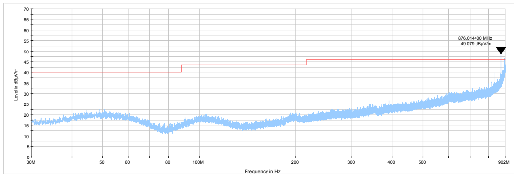
Plot 7.6.7 Radiated emission measurements from 30 to 902 MHz at the high carrier frequency
