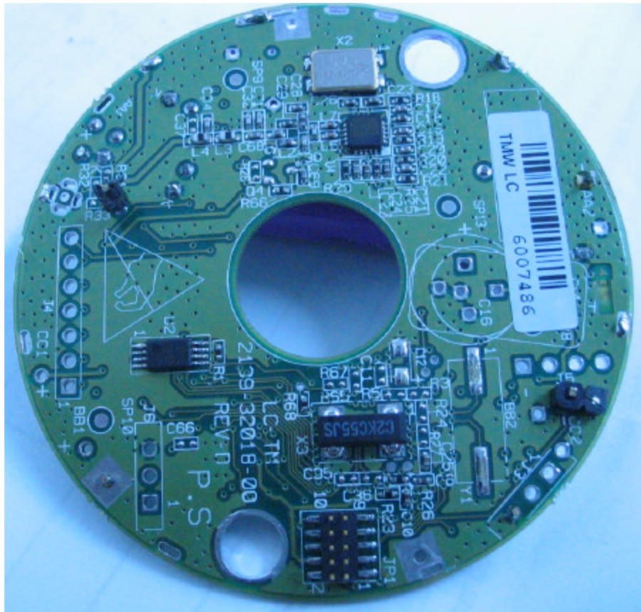
Photograph No.7 RF module PCB second side
