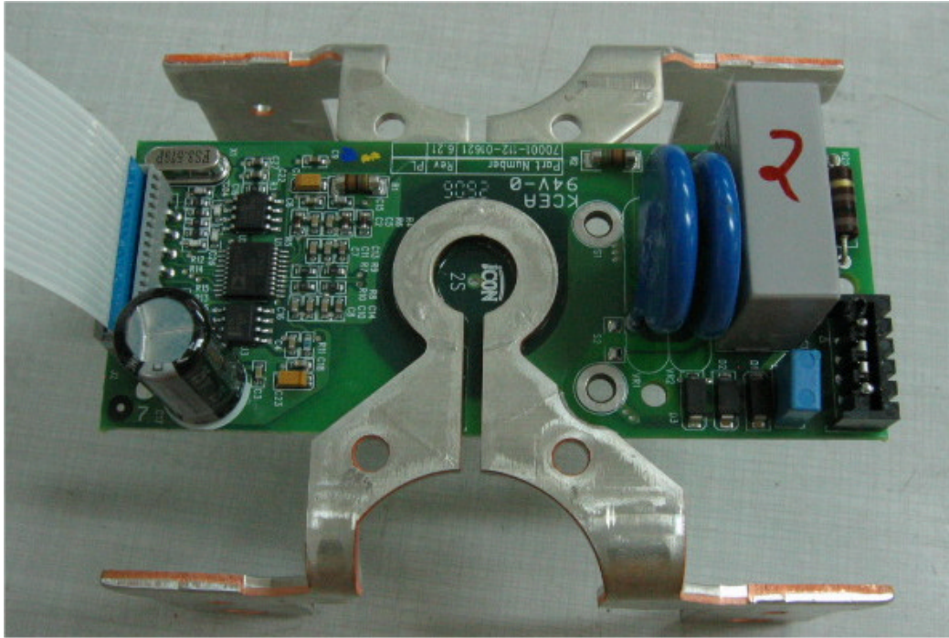
Photograph No.9 Sensor module PCB top view
