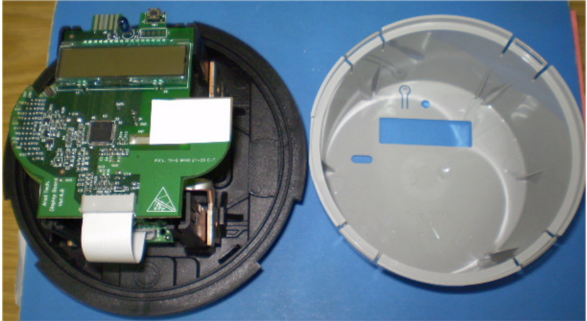
Photograph No.1 ICON240V internal view (antenna closed)
