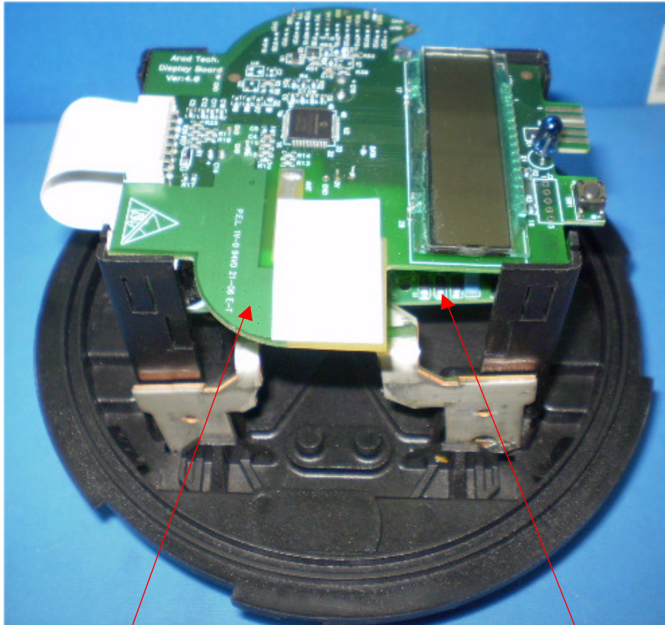
Photograph No.3 ICON240V internal side view
