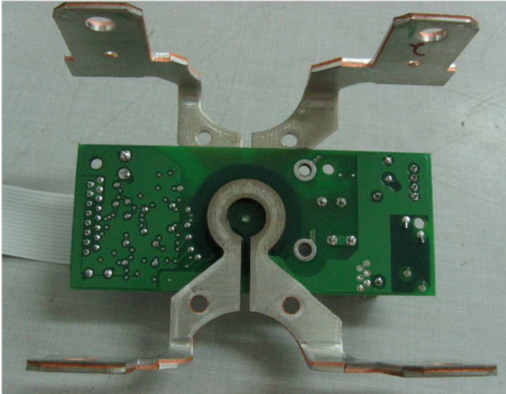
Photograph No.10 Sensor module PCB second side view
