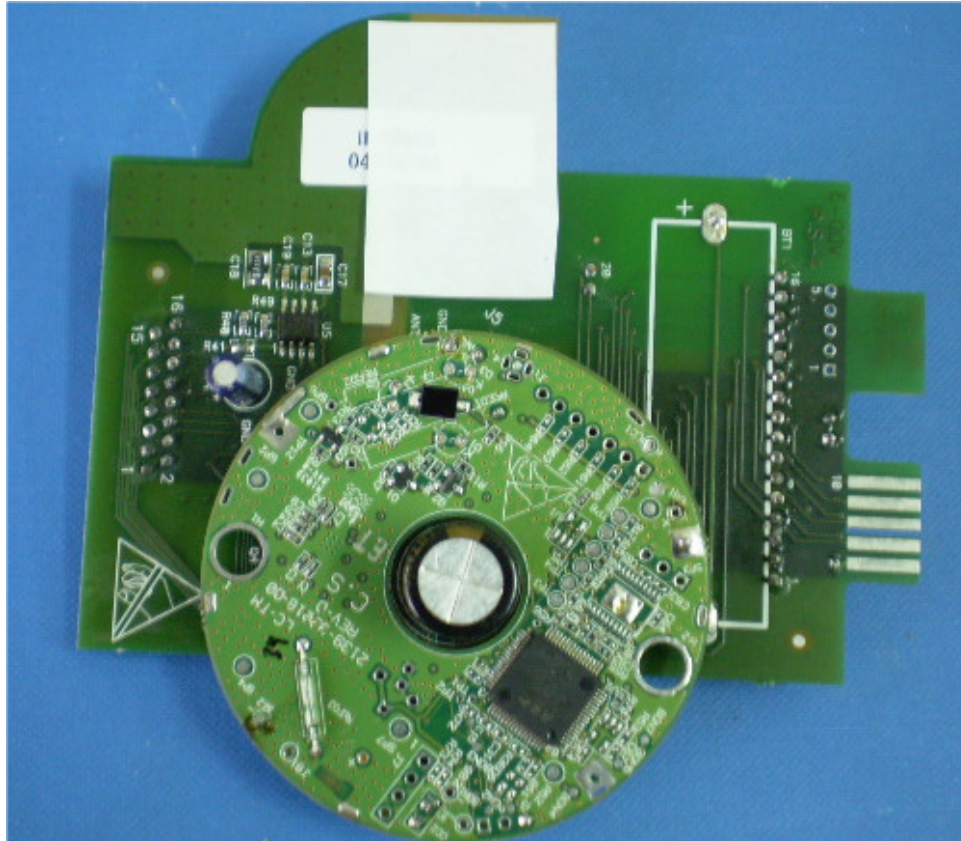
Photograph No.5 Display board view from the second side (antenna closed)
