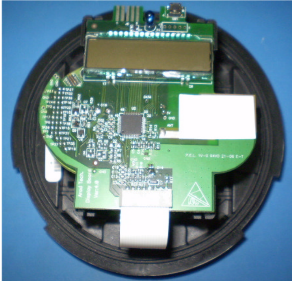
Photograph No.2 ICON240V internal view without cover
