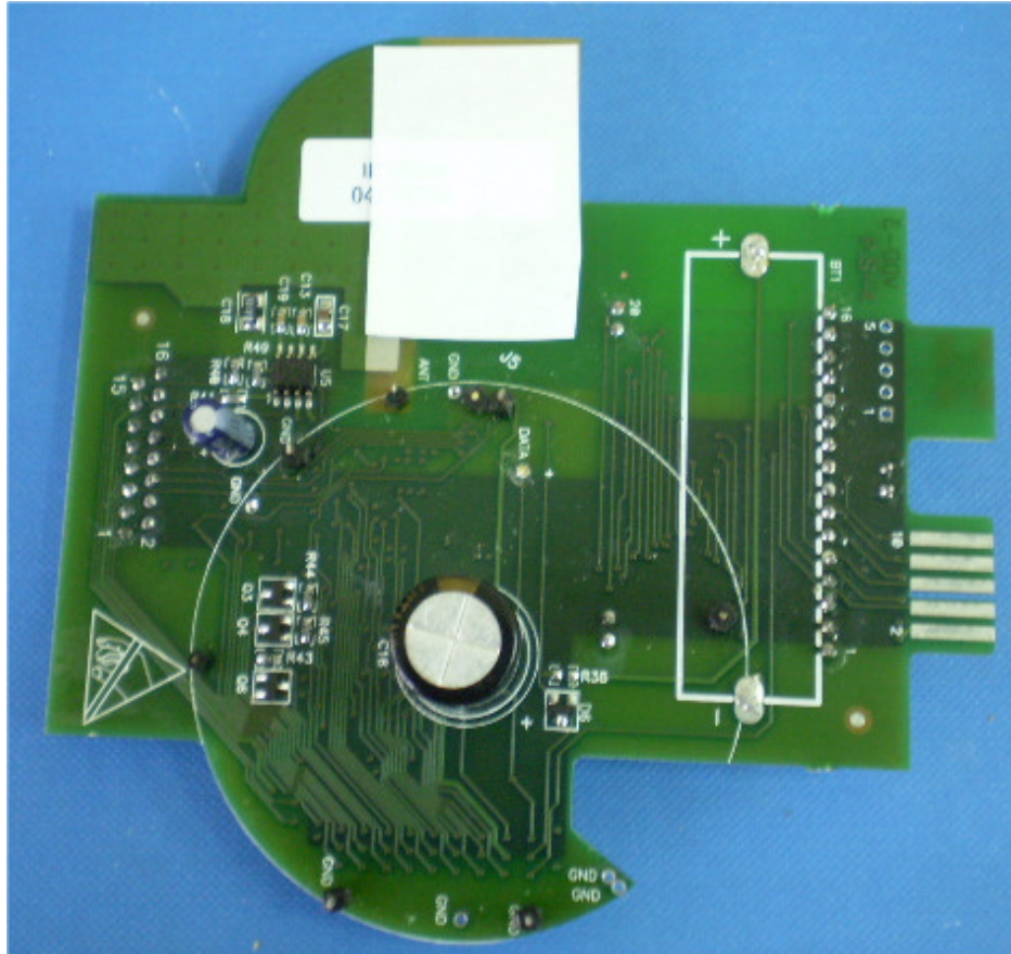
Photograph No.8 Display board view without RF module
