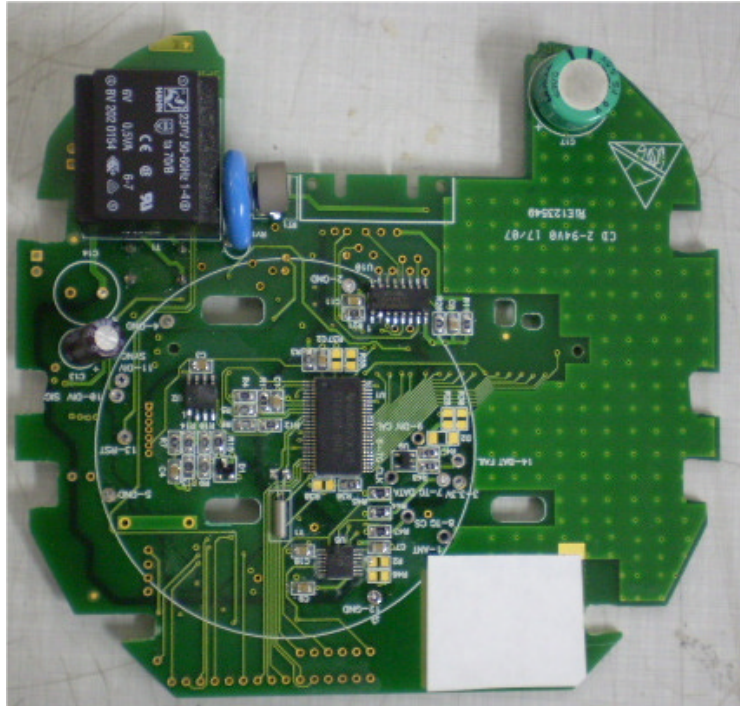
Photograph No.12 Display board view without RF module
