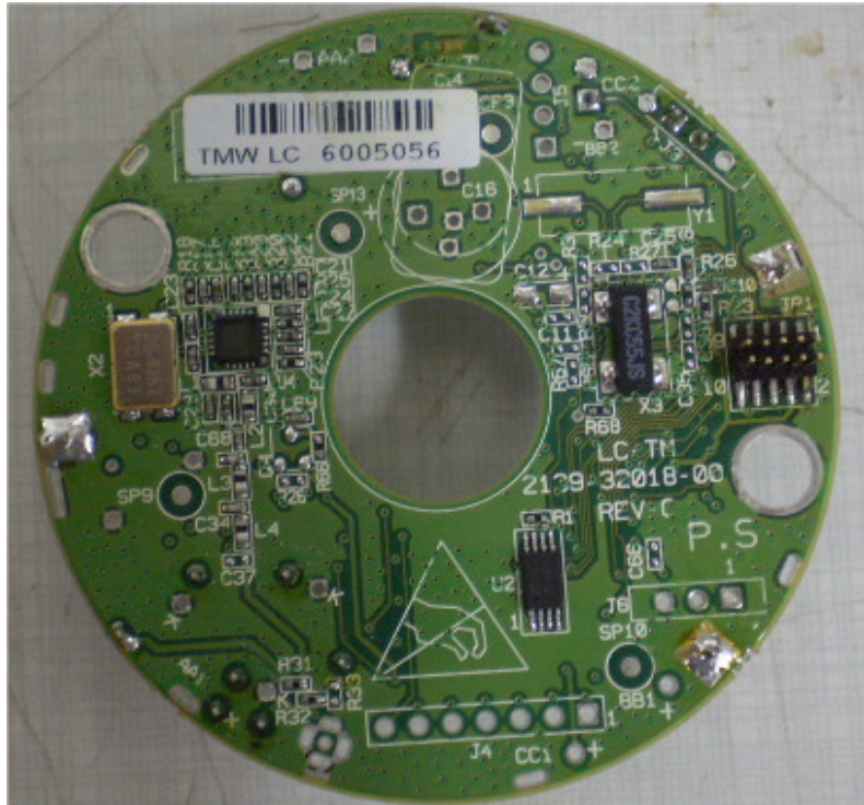
Photograph No.10 RF module
