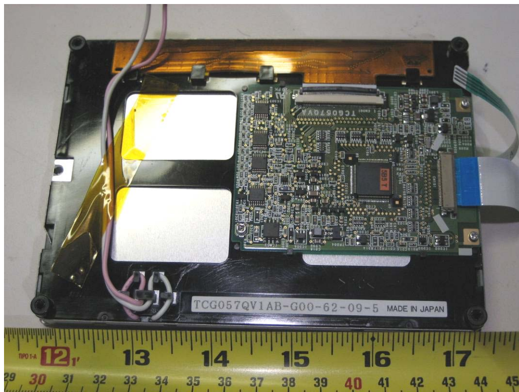
LCD Module Back View
