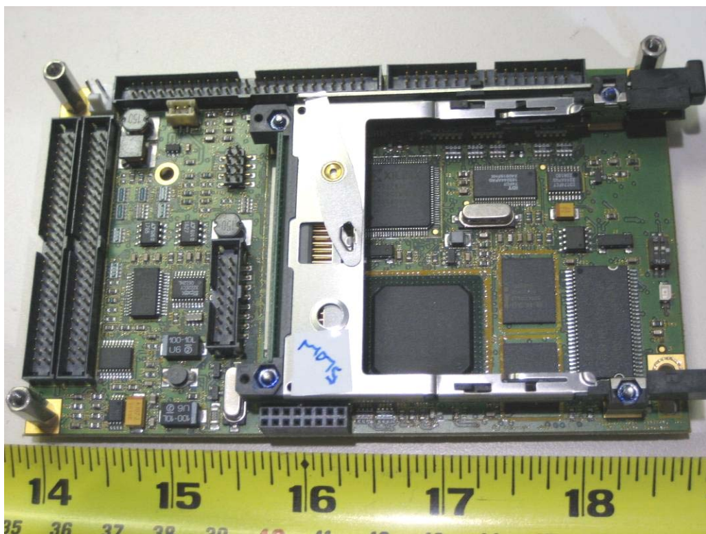
Daughter Card 1 Top View
