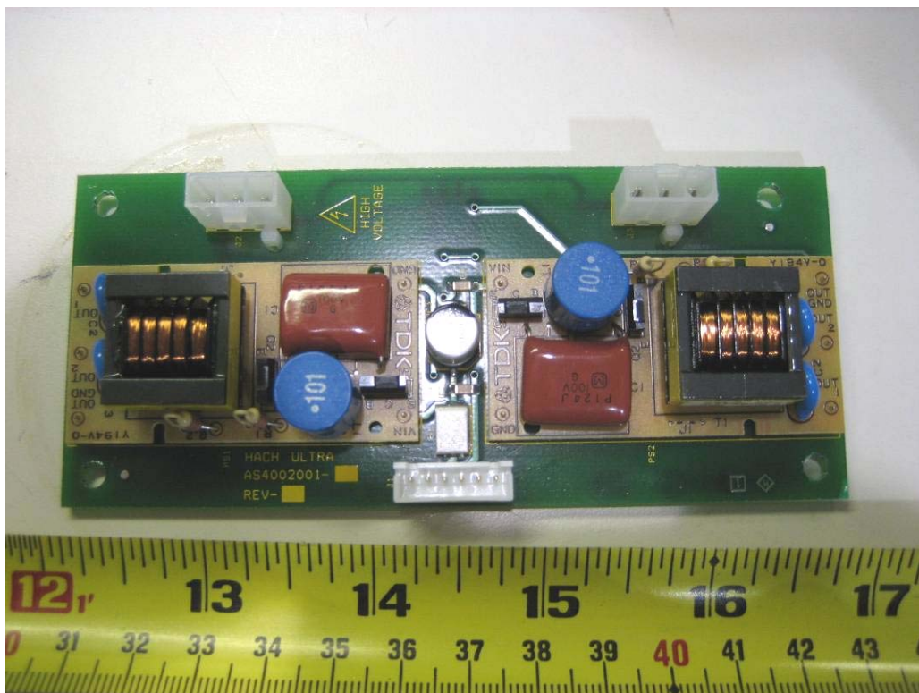
Voltage Regulator Board Top View
