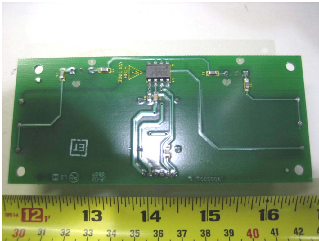
Voltage Regulator Board Bottom View
