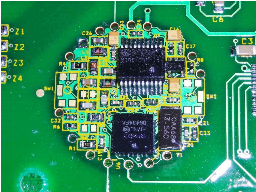
RFID Radio Module Bottom View
