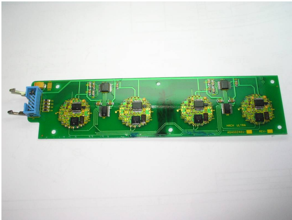
RFID Radio Module Top View
