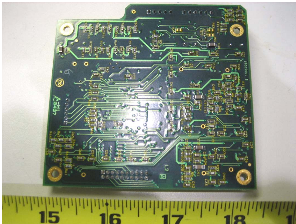
Daughter Card 1 Bottom View
