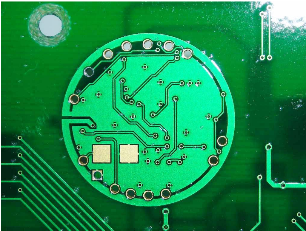
Antenna Close View
