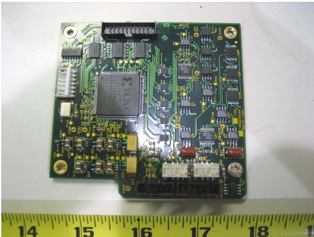
Daughter Card 2 Top View
