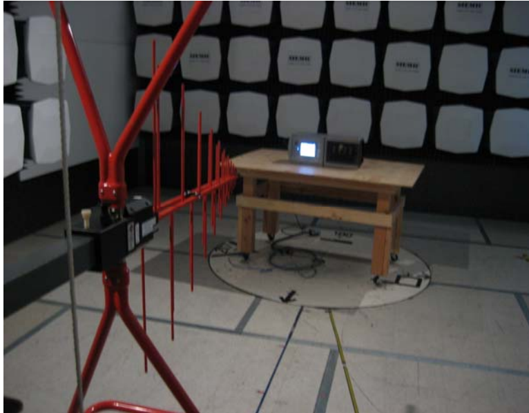
Radiated Emission Test Set-up Front View ( > 30 MHz )
