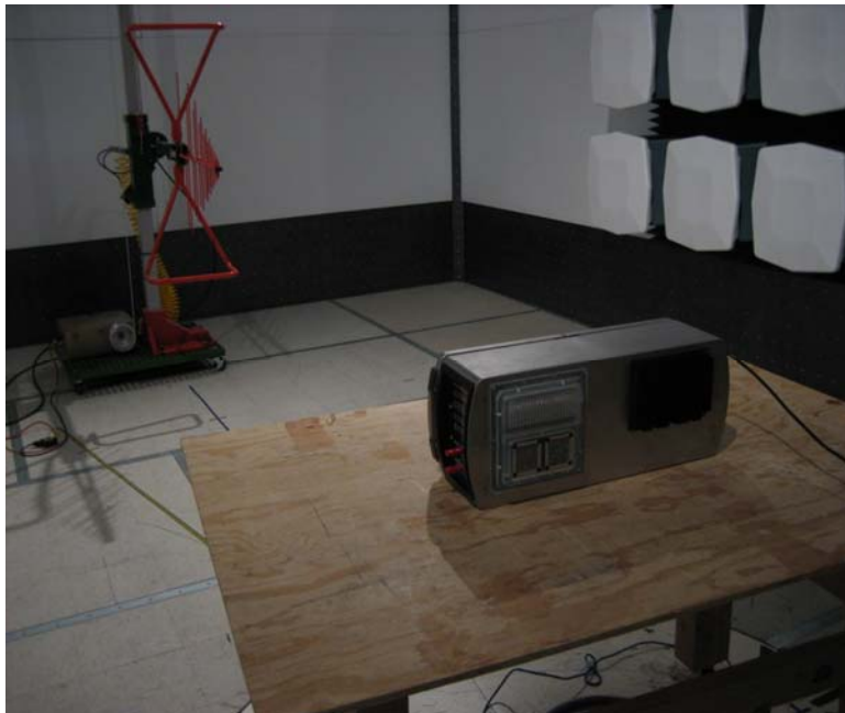
Radiated Emissions Test Set-up Rear View ( > 30 MHz )
