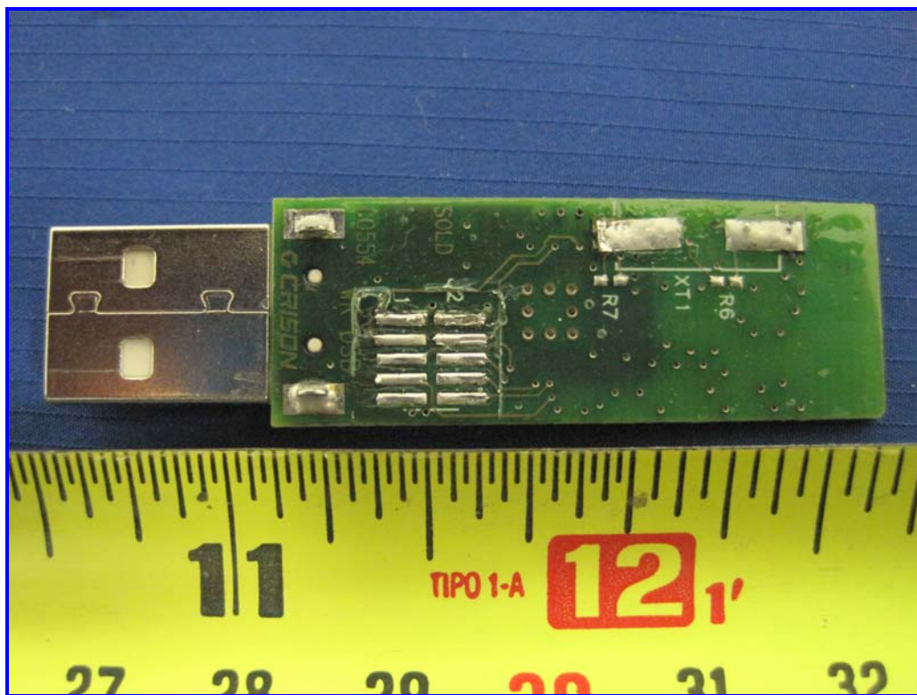
EUT – Main PCBA (C0554) with Radio Solder View
