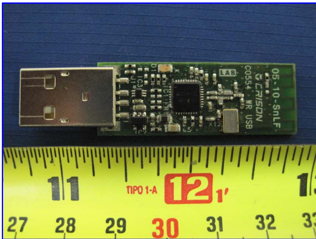
EUT – Main PCBA (C0554) with Radio Component View
