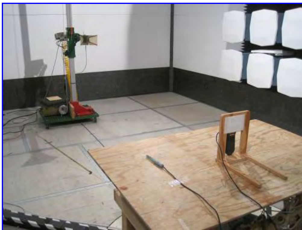
Radiated Emission, Host Model: sensION + MM 150 DL (Above 1GHz) – Rear View
