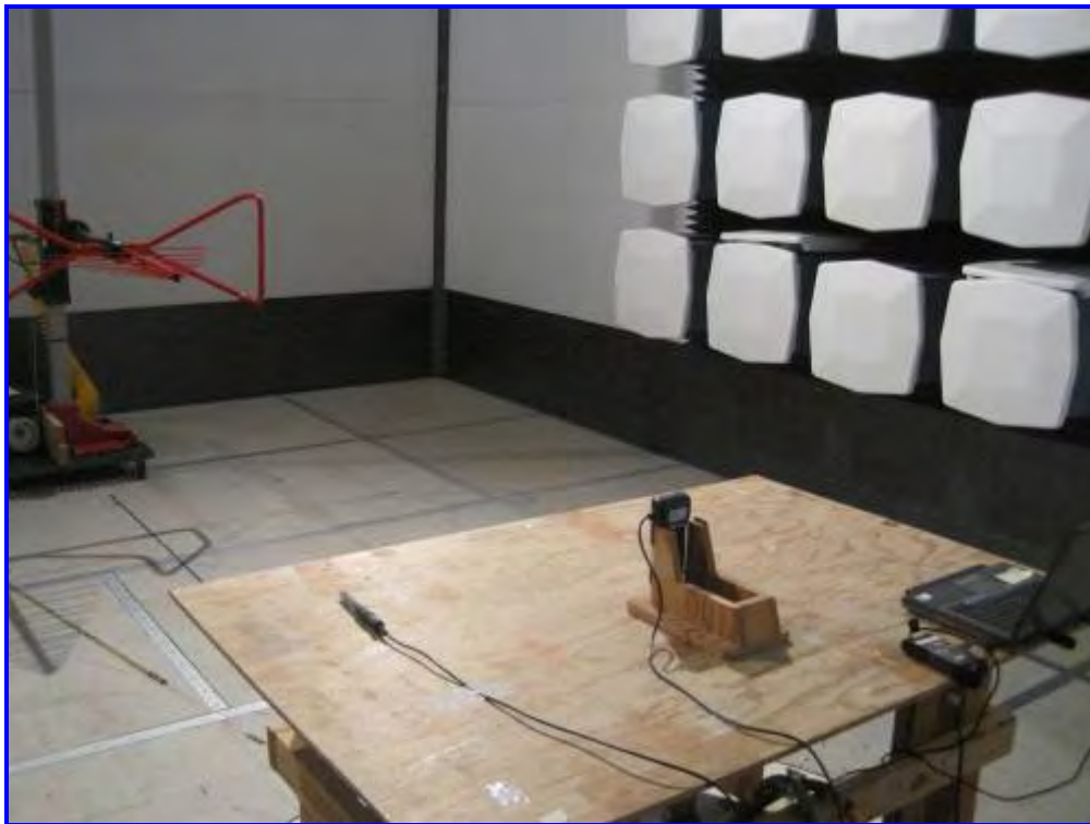
Radiated Emission, Host Model: sensION + DO 6 DL (30MHz - 1GHz) – Rear View
