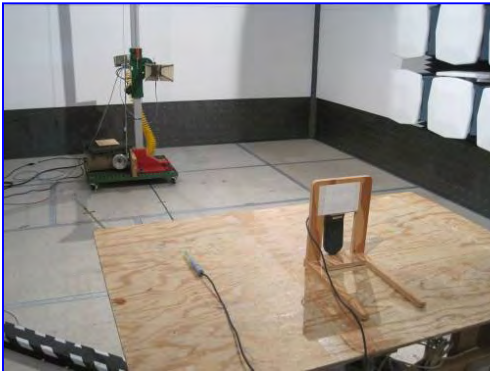
Radiated Emission, Host Model: sensION + MM 110 DL (Above 1GHz) – Rear View
