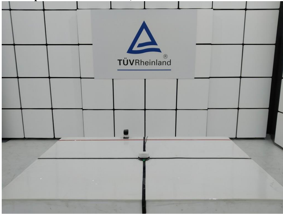
Picture 2: Test setup for Radiated Emission; 30 MHz- 1000 MHz
