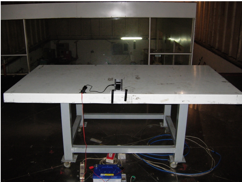
Back View of Radiated Test - Car Charger
