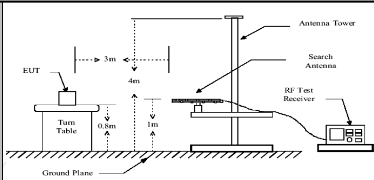
Above 1GHz
