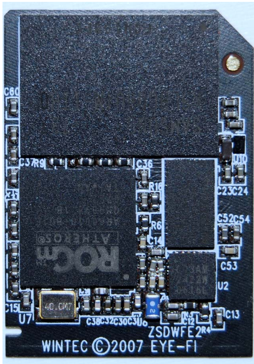
Figure 1: Eye-Fi Card internal Photo (front)
