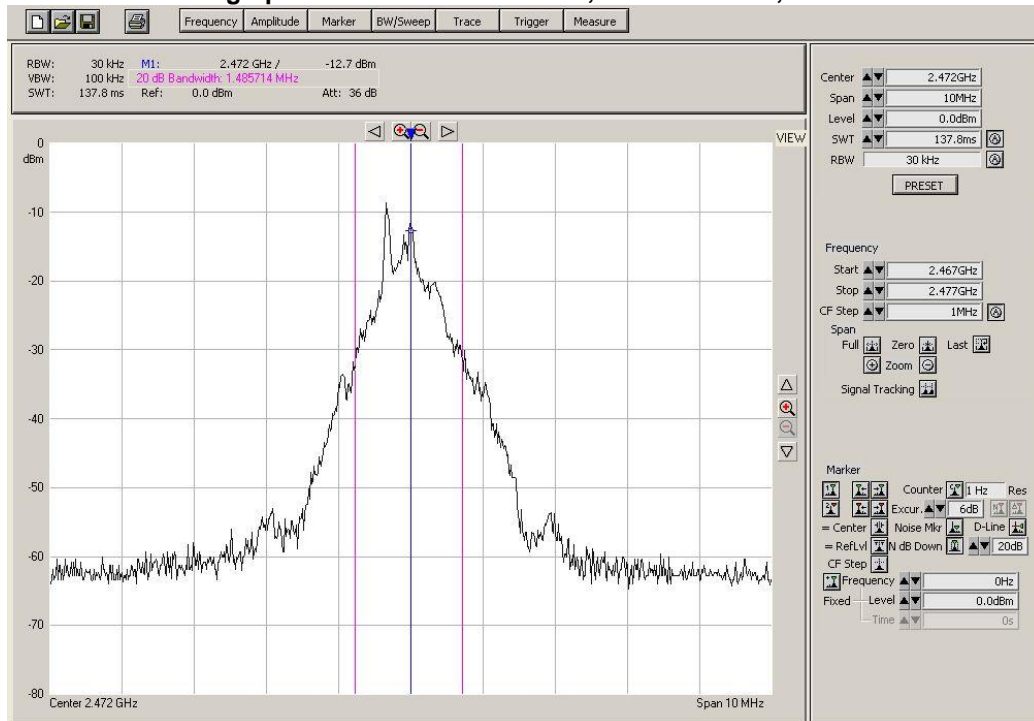
Figure 4 – Result data graph shows 20 dB bandwidth, CF = 2.472GHz, BW = 1.49MHz
