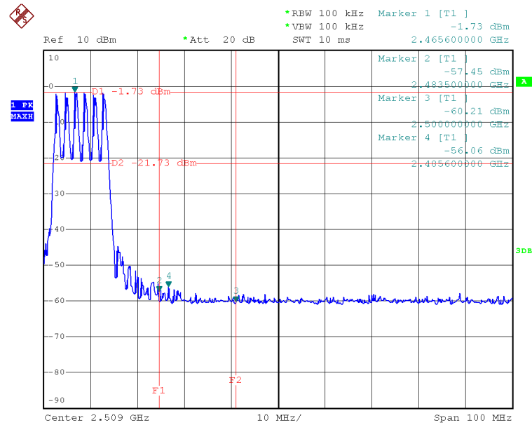
Figure 9 – Result data graph shows the frequency of highest channel.
