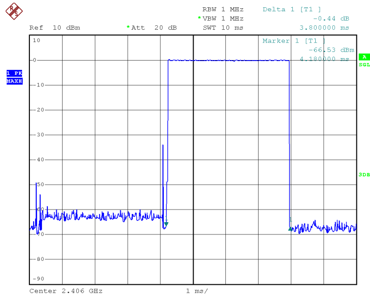
Figure 7 – Result data graph zooms into detail, one pulse period is 3.8ms.
