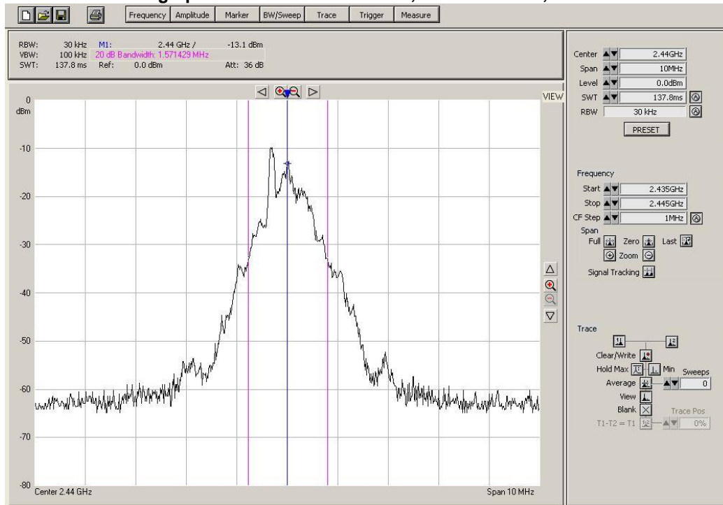
Figure 3 – Result data graph shows 20 dB bandwidth, CF = 2.440GHz, BW = 1.57MHz
