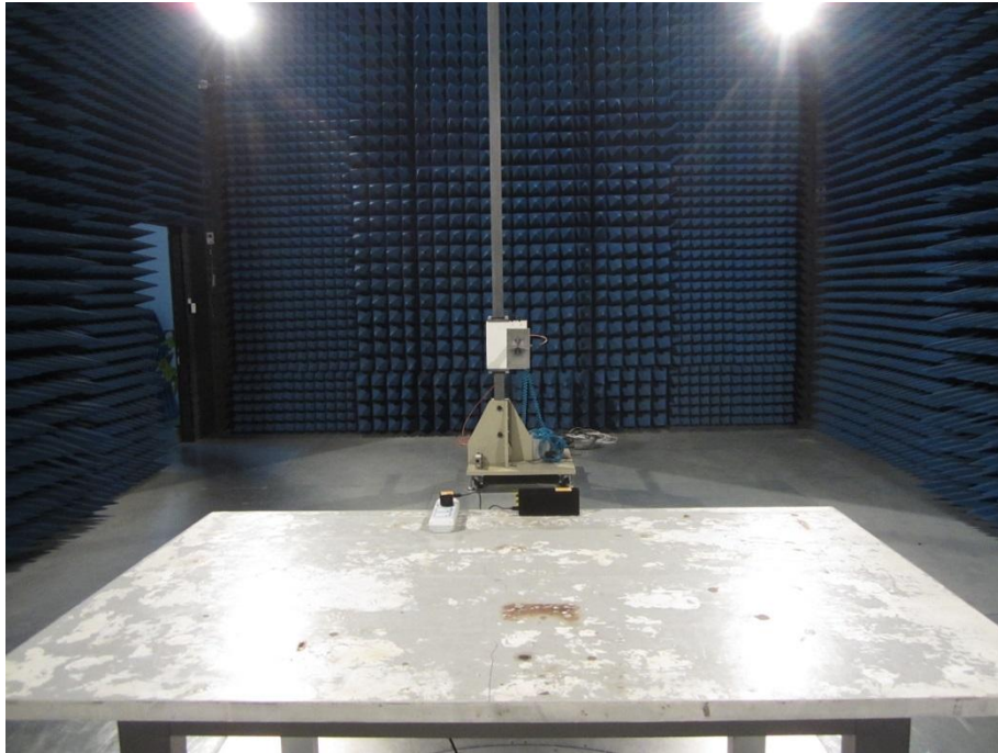
Figure 3 Radiated emission
