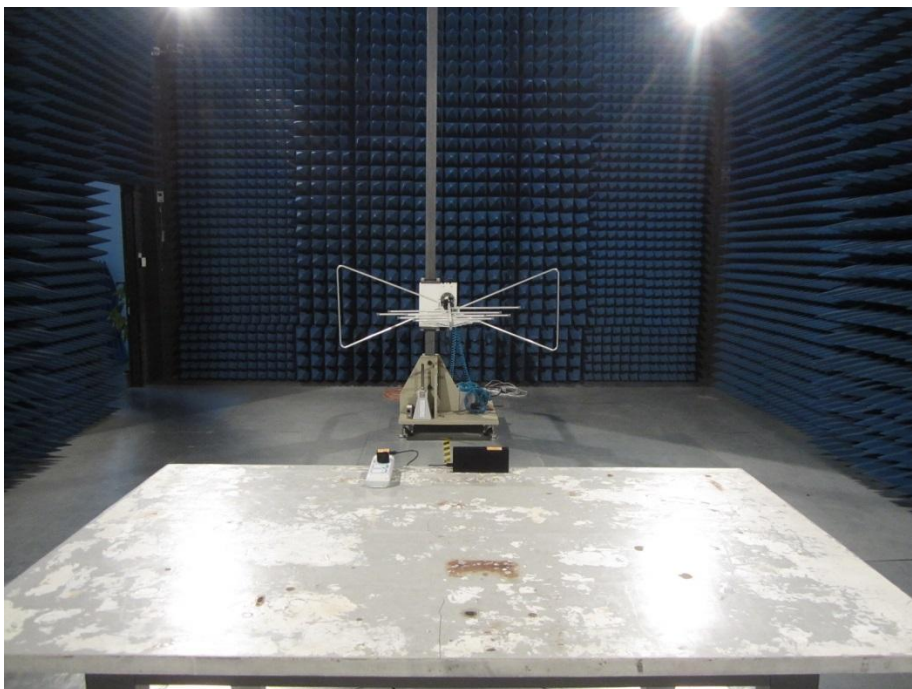
Figure 2 Radiated emission
