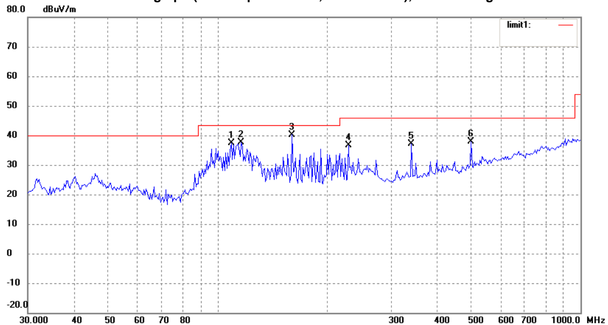
Radiated emission data graph (Vertical polarization, 30MHz-1GHz), Transmitting Mode
