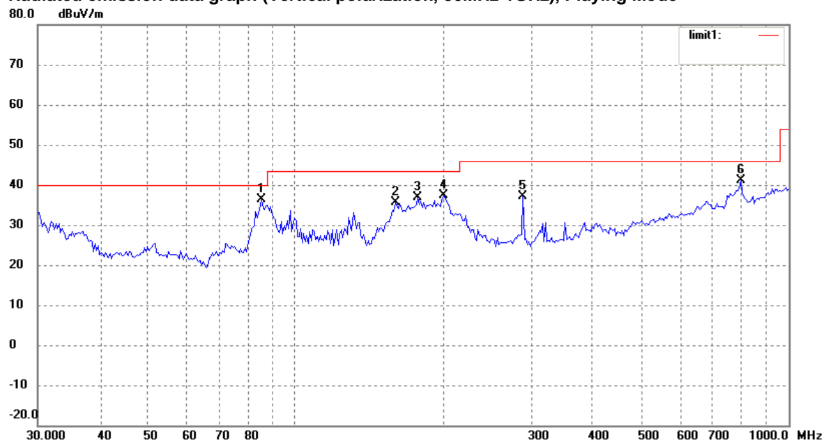
Radiated emission data graph (Vertical polarization, 30MHz-1GHz), Playing Mode
