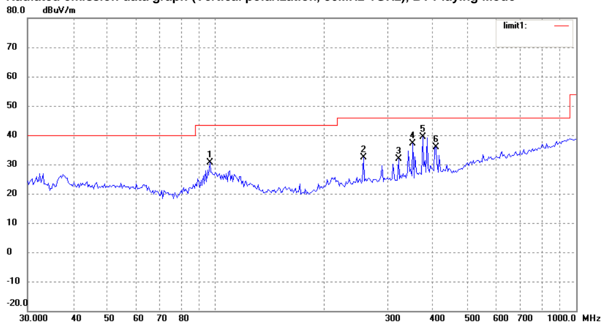
Radiated emission data graph (Vertical polarization, 30MHz-1GHz), BT Playing Mode
