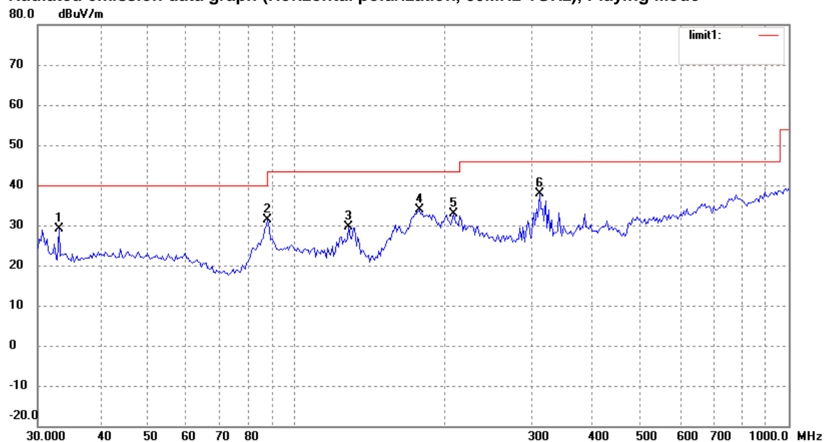
Radiated emission data graph (Horizontal polarization, 30MHz-1GHz), Playing Mode
