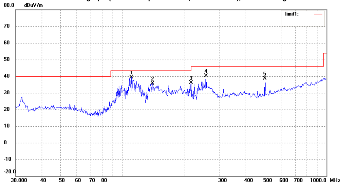
Radiated emission data graph (Horizontal polarization, 30MHz-1GHz), Transmitting Mode
