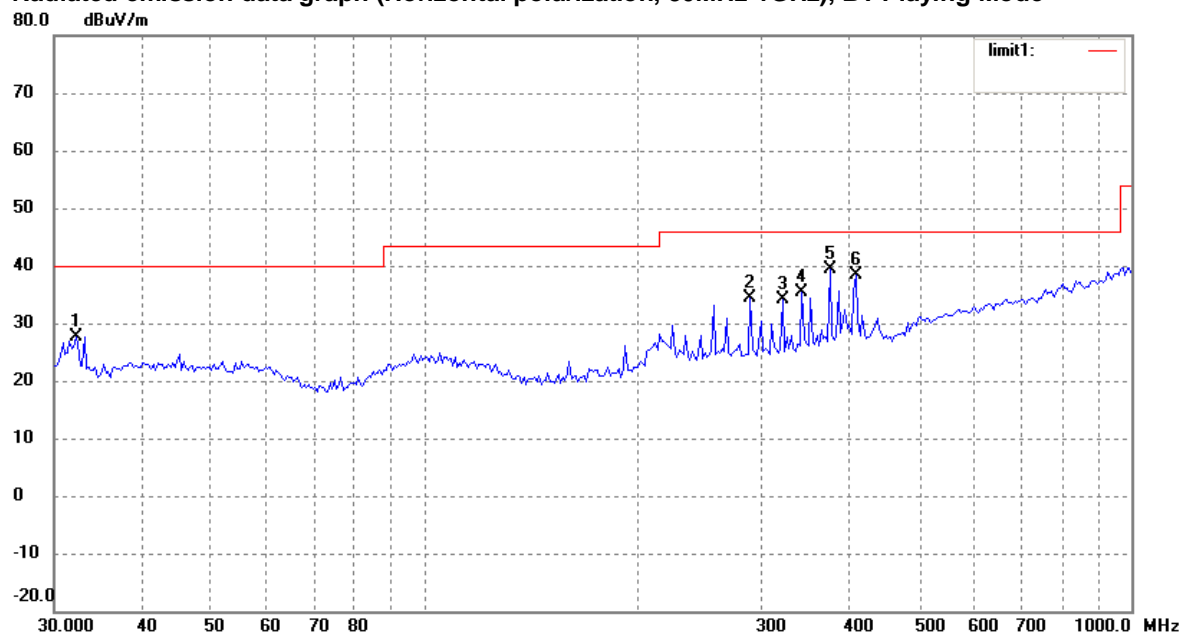
Radiated emission data graph (Horizontal polarization, 30MHz-1GHz), BT Playing Mode
