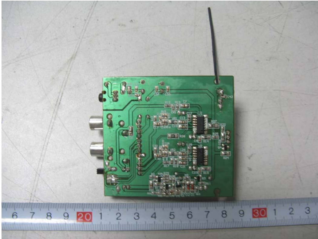
EUT- Main Board Component Bottom View
