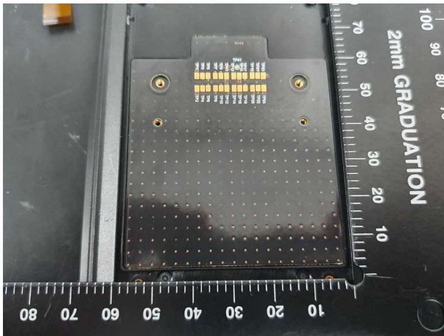
Sub board 3
