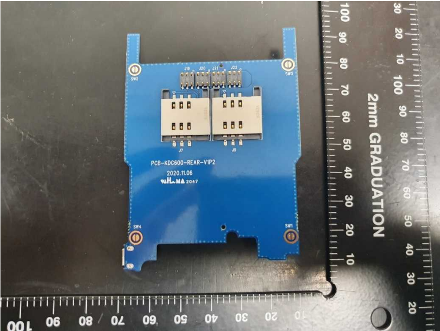
Sub board 1 - Front Top
