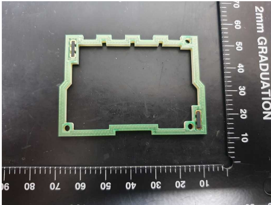
Ant board 1 - Front Top
