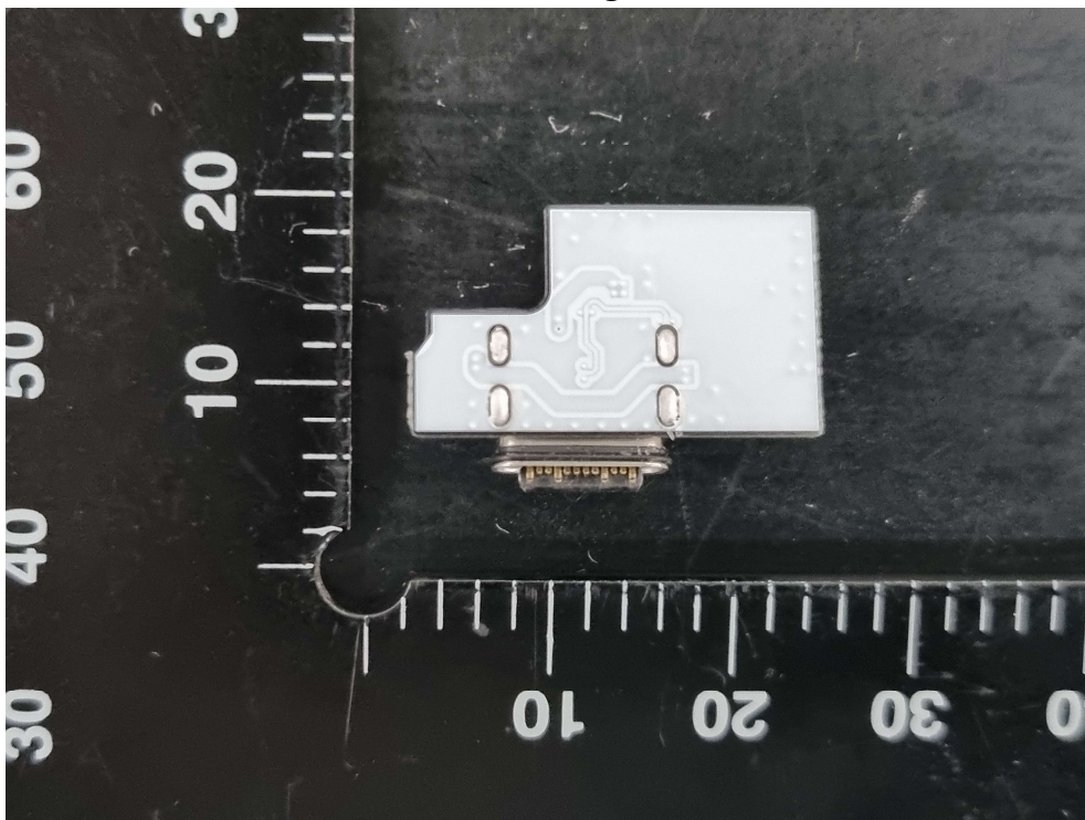
Sub Board(Charger, Rear)
