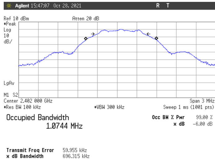
Figure 1. Plot of the 6dB Bandwidth & Occupied Bandwidth (99%)
