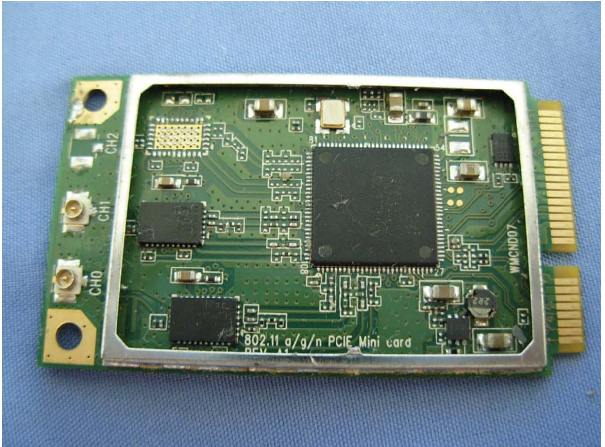
(24) EUT Photo (5G MB)
