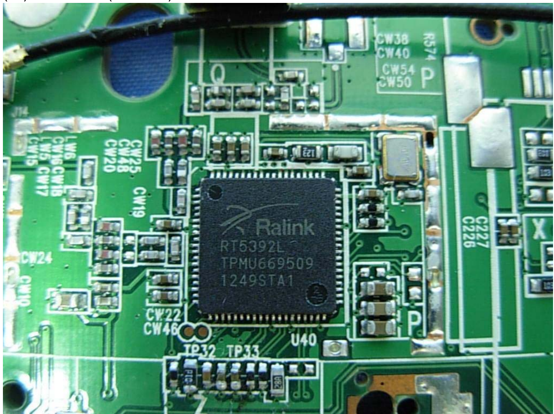
(19) EUT Photo (2.4G MB)
