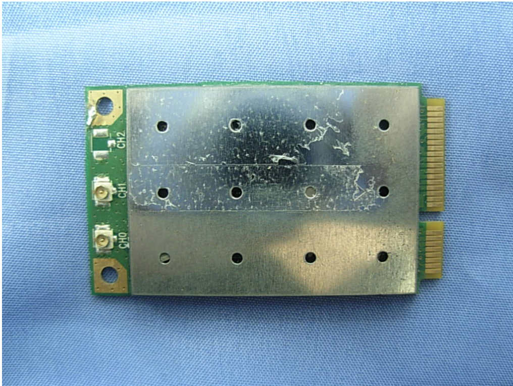
(5) EUT Photo (Module Model: WMC-ND07D)
