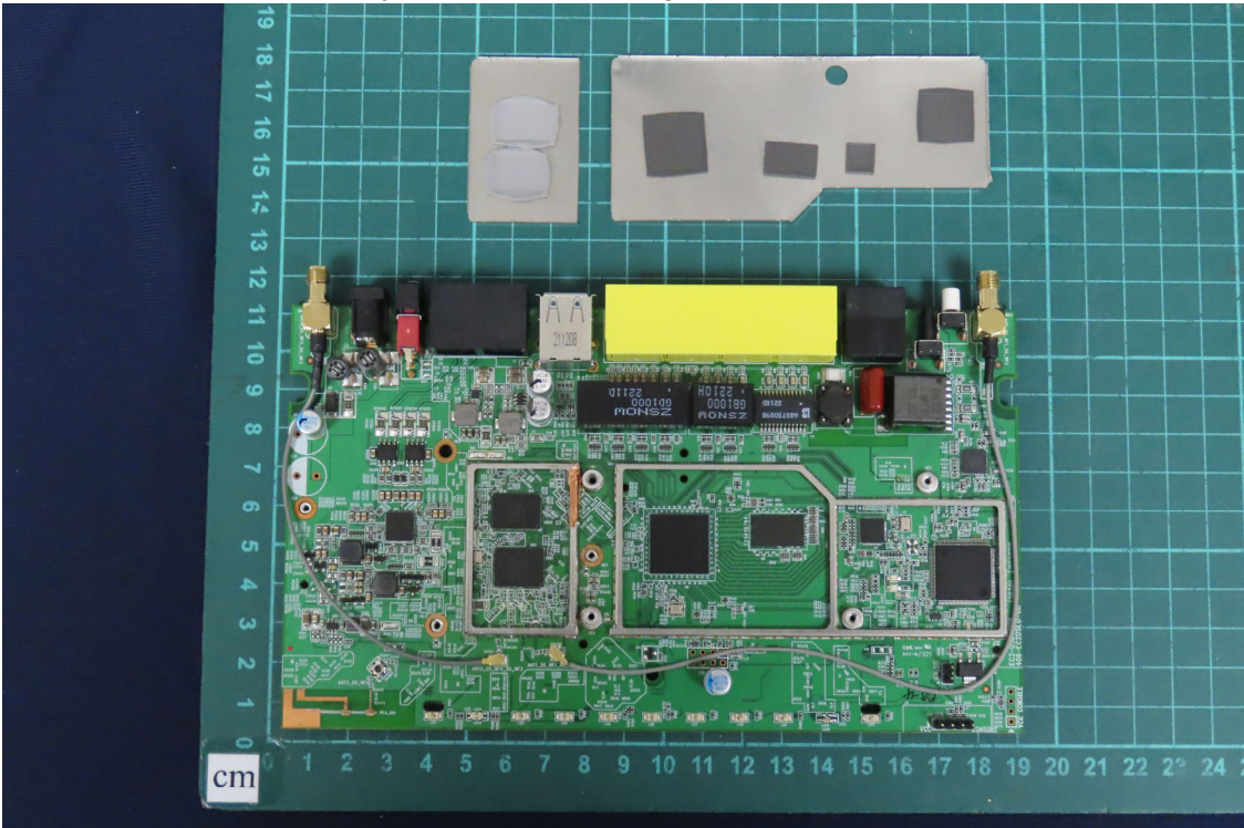
(7) EUT Photo - Trademark: DrayTek, Model No.: Vigor2767Vax
