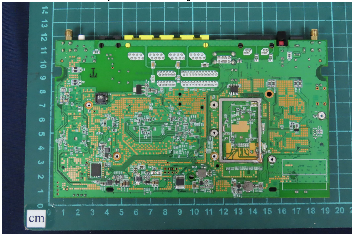
(15) EUT Photo - Trademark: DrayTek, Model No.: Vigor2767Vax
