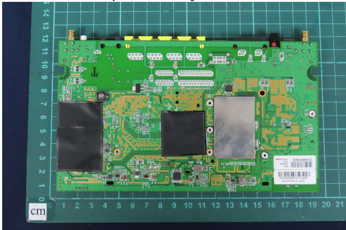
(13) EUT Photo - Trademark: DrayTek, Model No.: Vigor2767Vax
