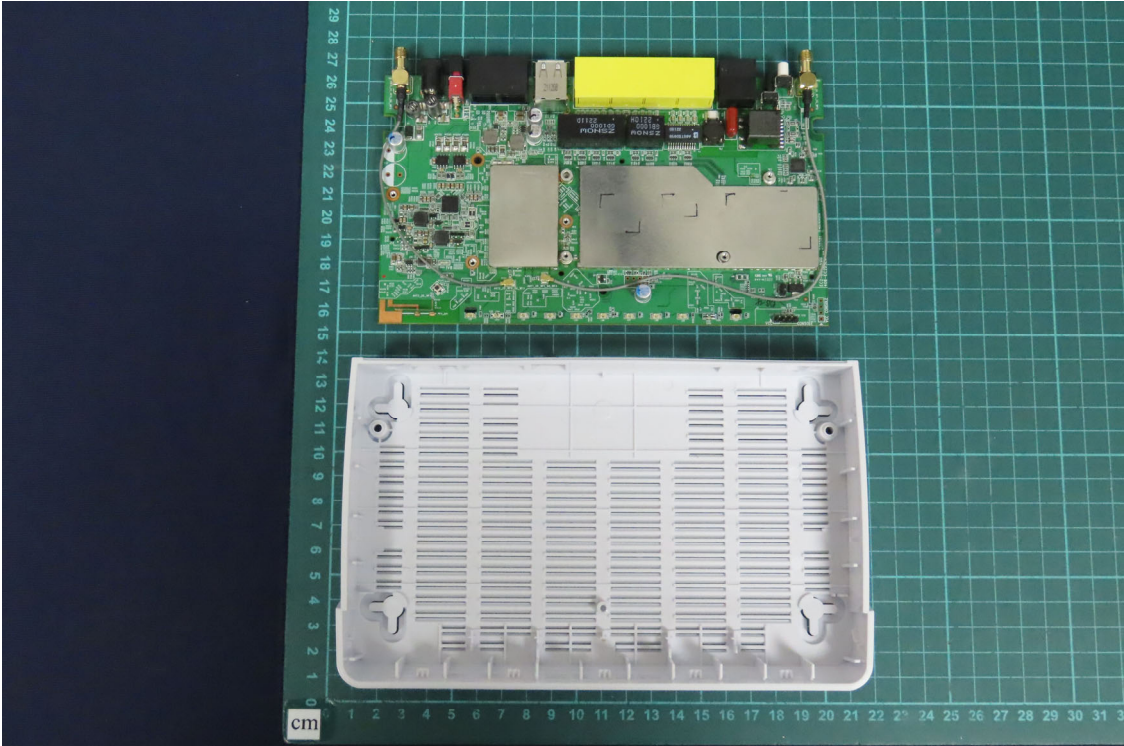
(5) EUT Photo - Trademark: DrayTek, Model No.: Vigor2767Vax
