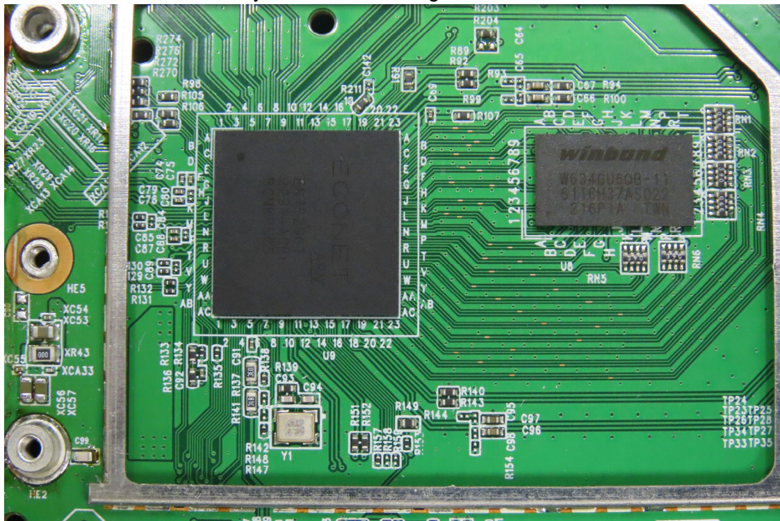
(10) EUT Photo - Trademark: DrayTek, Model No.: Vigor2767Vax
