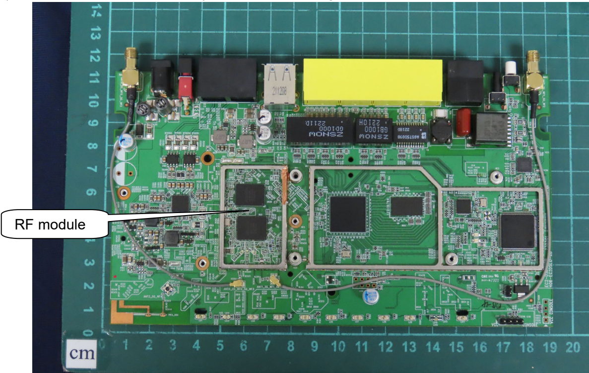
(8) EUT Photo - Trademark: DrayTek, Model No.: Vigor2767Vax
