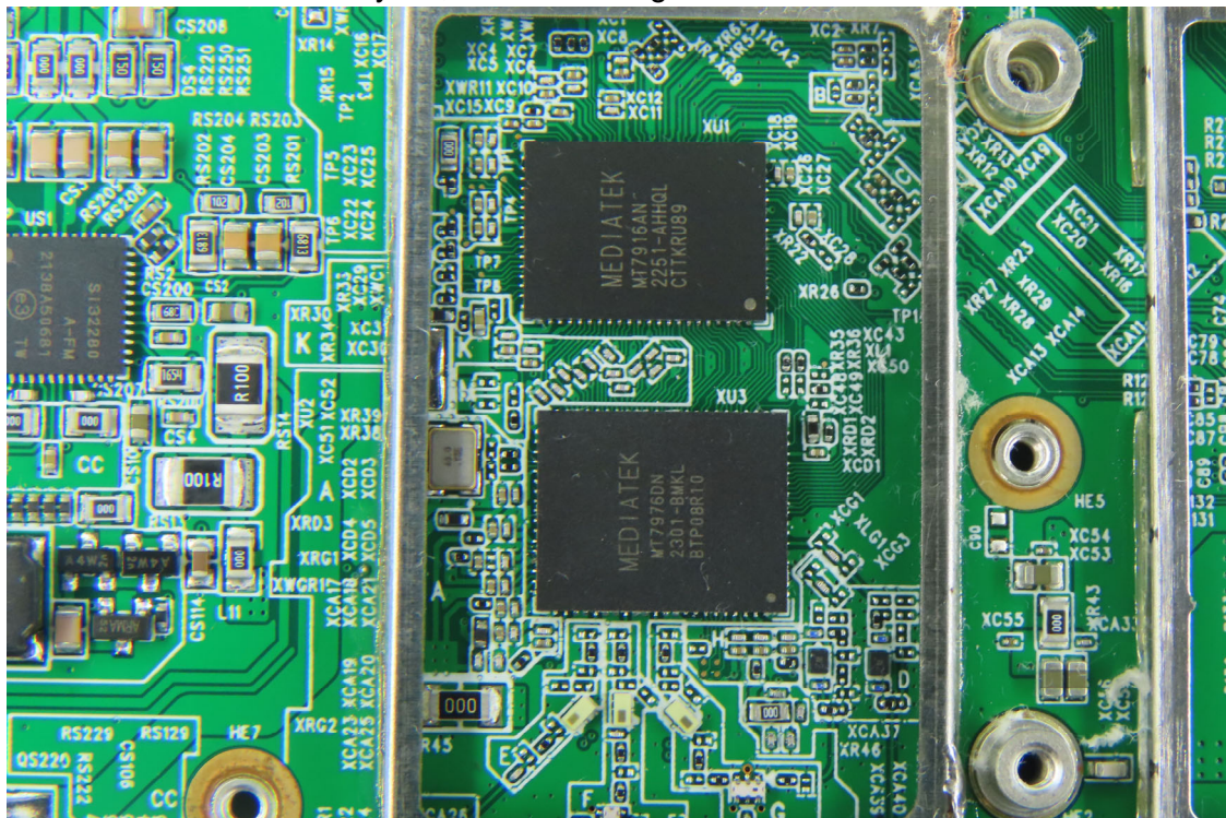
(24) EUT Photo - Trademark: DrayTek, Model No.: Vigor2136Vax
