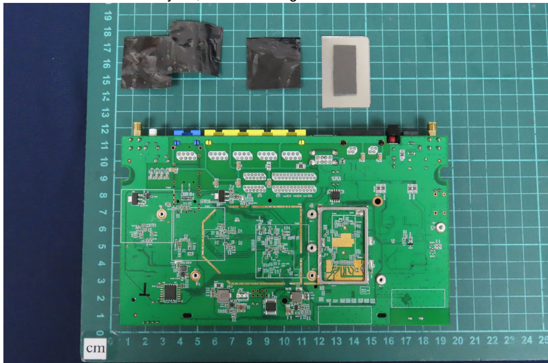
(29) EUT Photo - Trademark: DrayTek, Model No.: Vigor2136Vax
