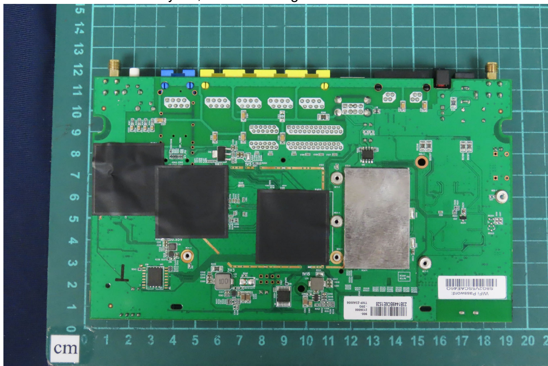
(28) EUT Photo - Trademark: DrayTek, Model No.: Vigor2136Vax
