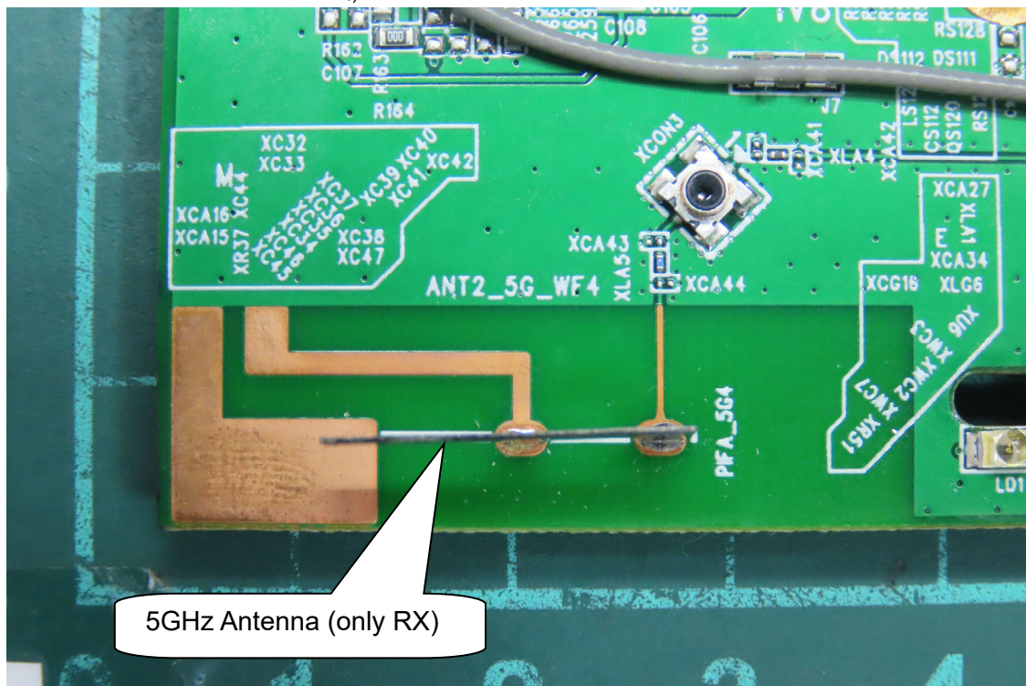
(27) EUT Photo - Trademark: INPAQ, Model No.: RFMTA160800NN5B002
