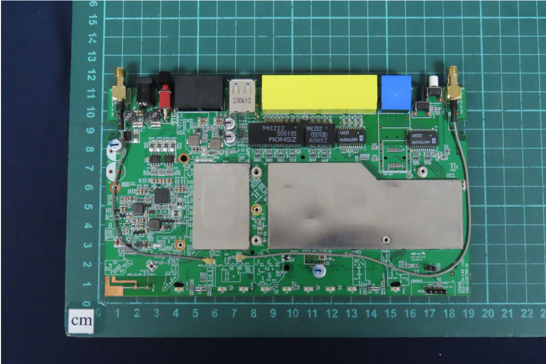
(21) EUT Photo - Trademark: DrayTek, Model No.: Vigor2136Vax
