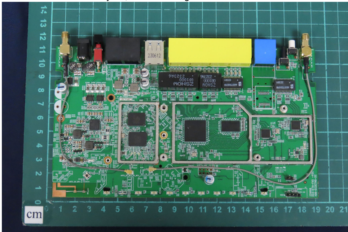
(23) EUT Photo - Trademark: DrayTek, Model No.: Vigor2136Vax
