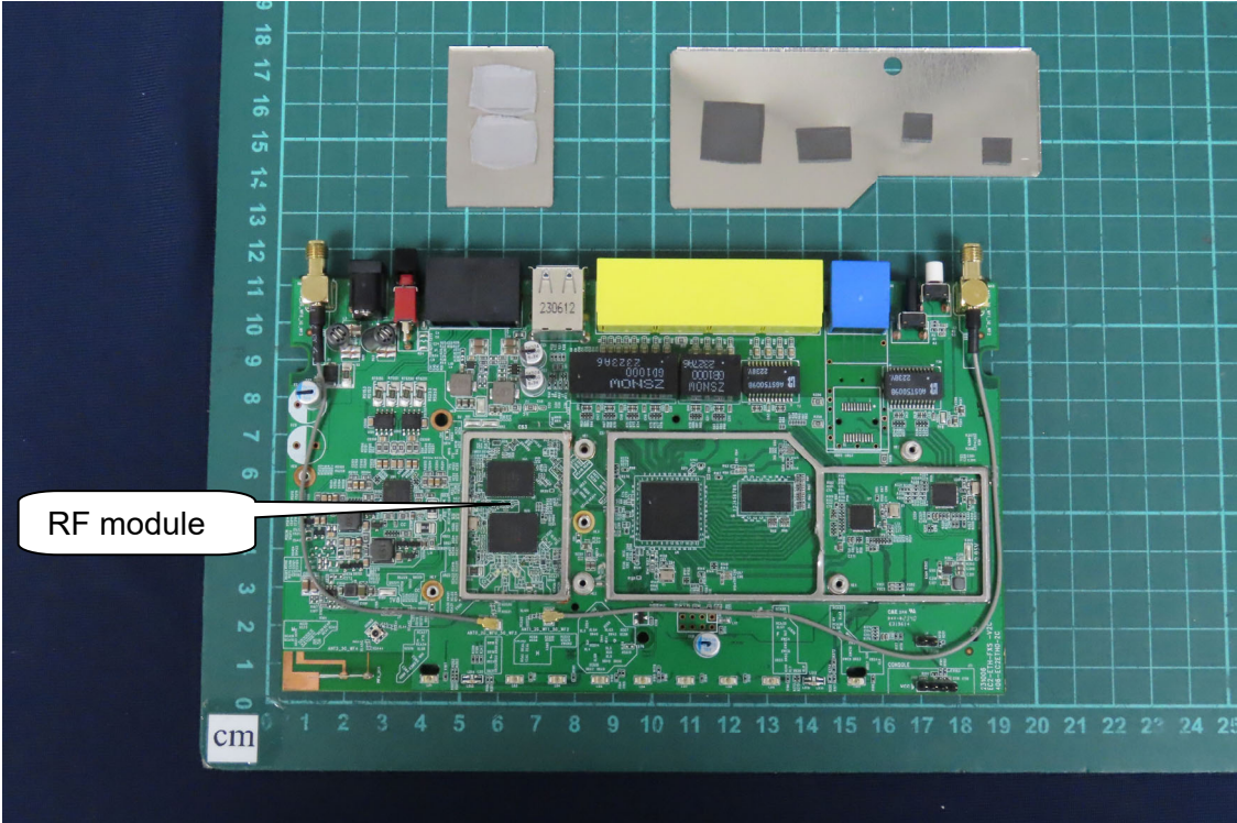
(22) EUT Photo - Trademark: DrayTek, Model No.: Vigor2136Vax
