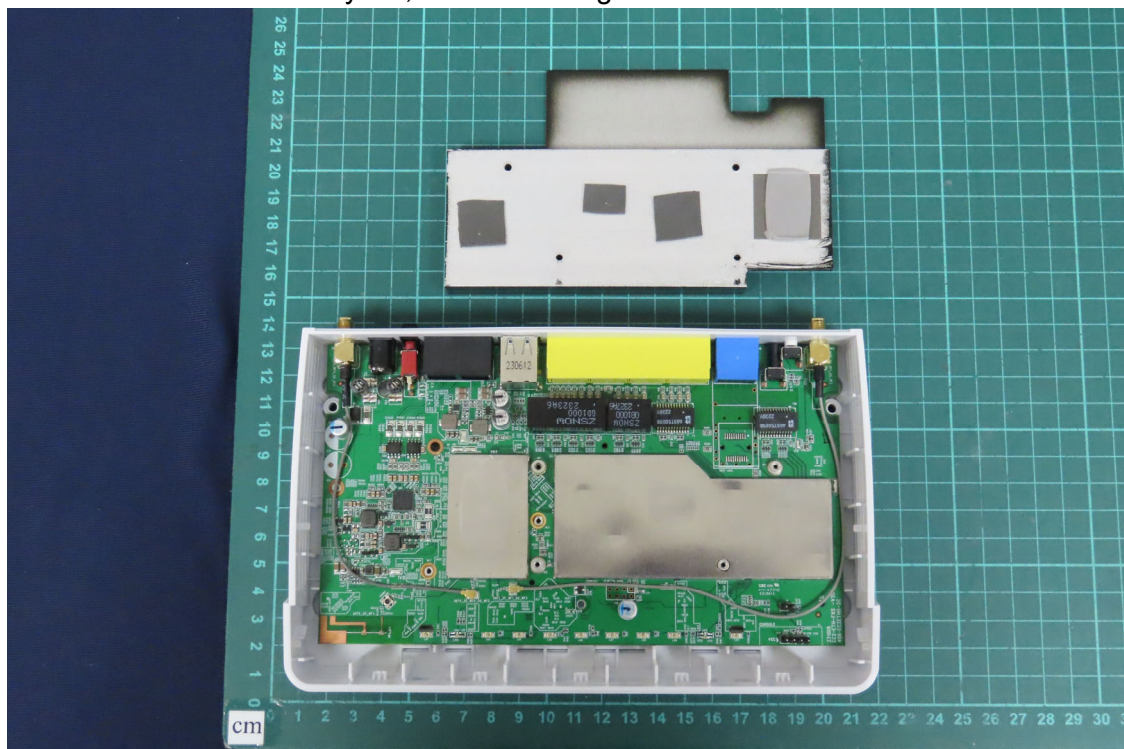
(18) EUT Photo - Trademark: DrayTek, Model No.: Vigor2136Vax
