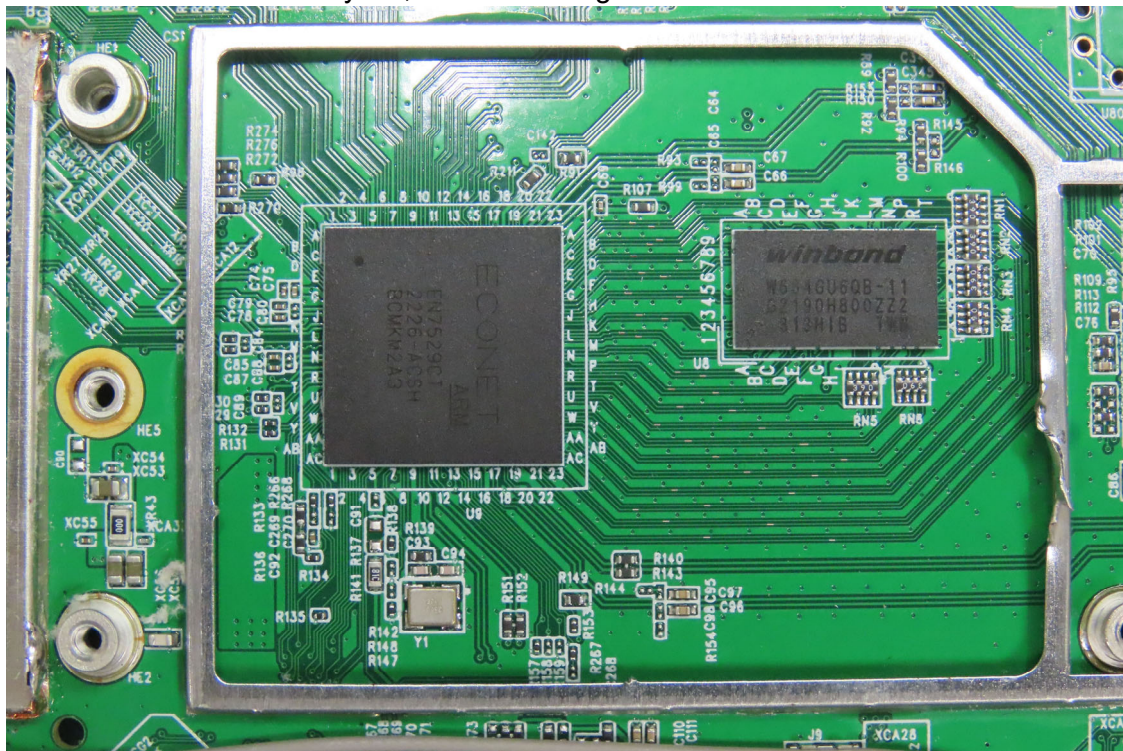
(25) EUT Photo - Trademark: DrayTek, Model No.: Vigor2136Vax
