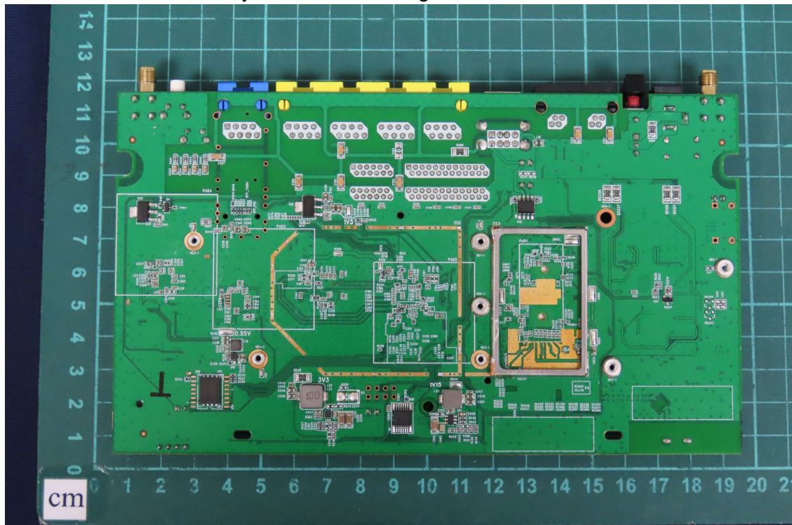
(30) EUT Photo - Trademark: DrayTek, Model No.: Vigor2136Vax
