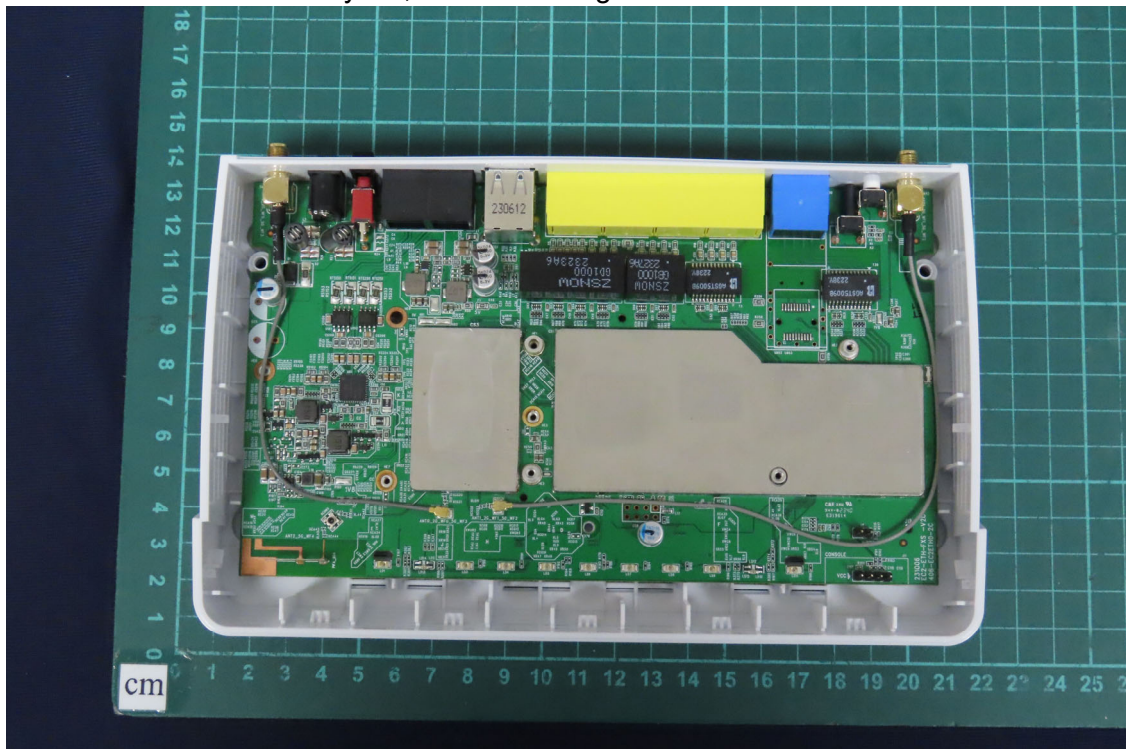
(19) EUT Photo - Trademark: DrayTek, Model No.: Vigor2136Vax
