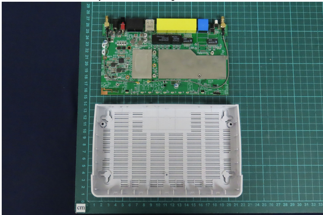
(20) EUT Photo - Trademark: DrayTek, Model No.: Vigor2136Vax
