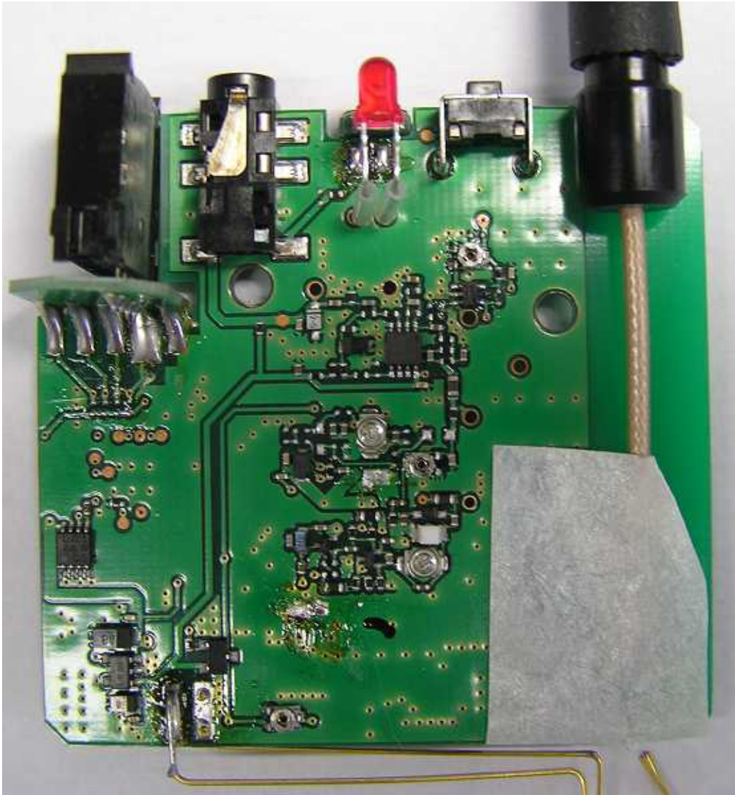
Transmitter PCB(top) without shield case
