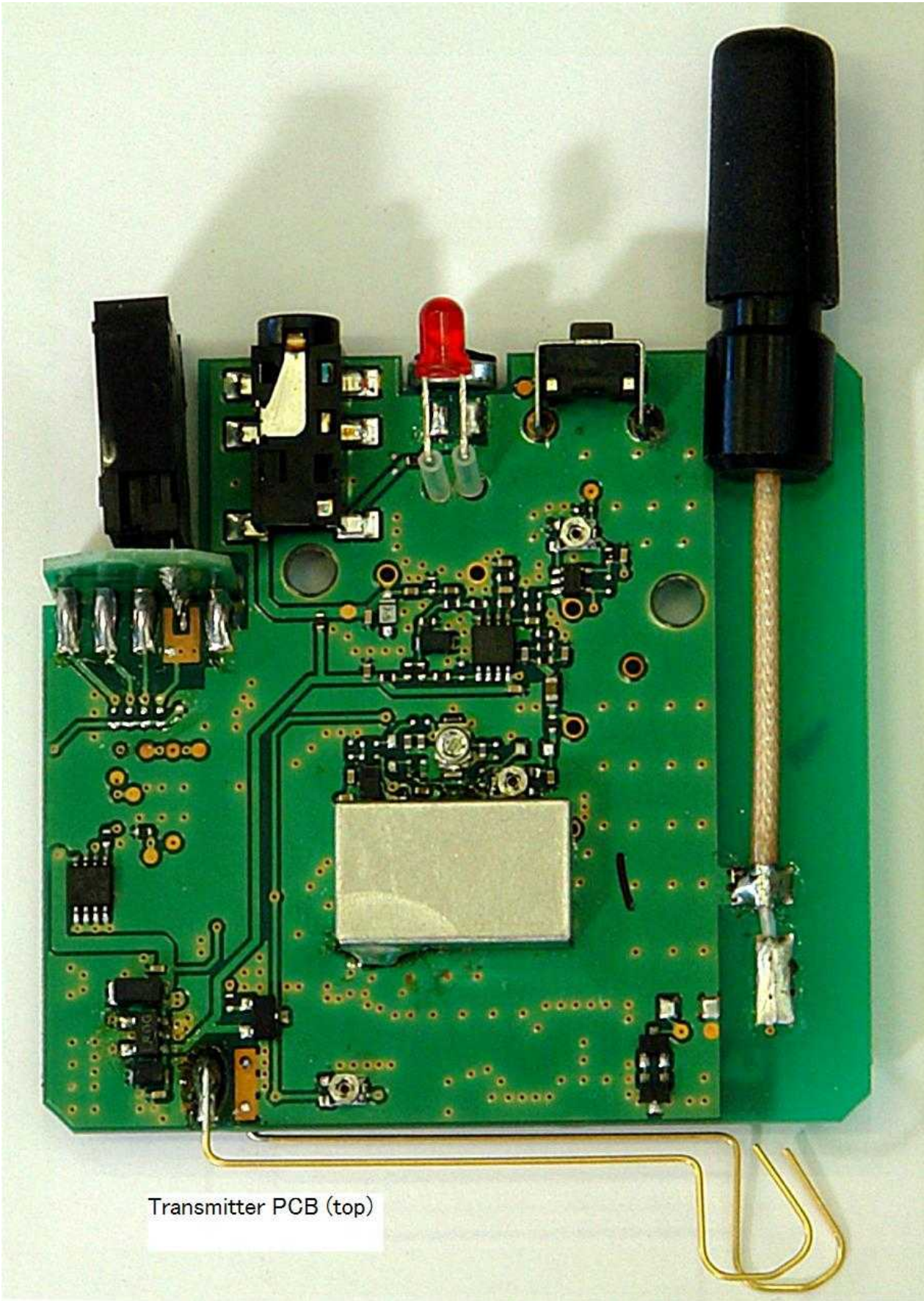
Transmitter PCB (top)
