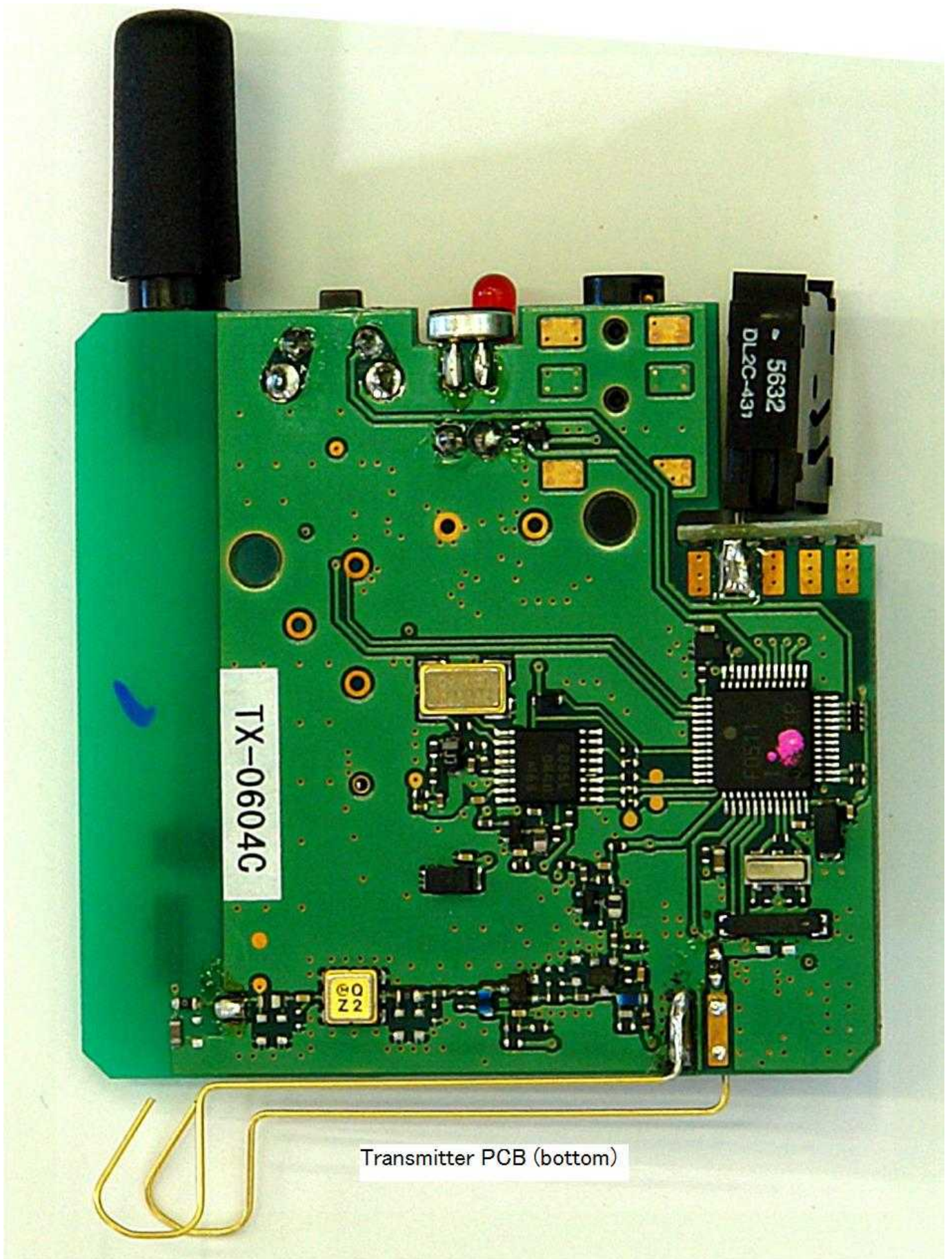
Transmitter PCB (bottom)
