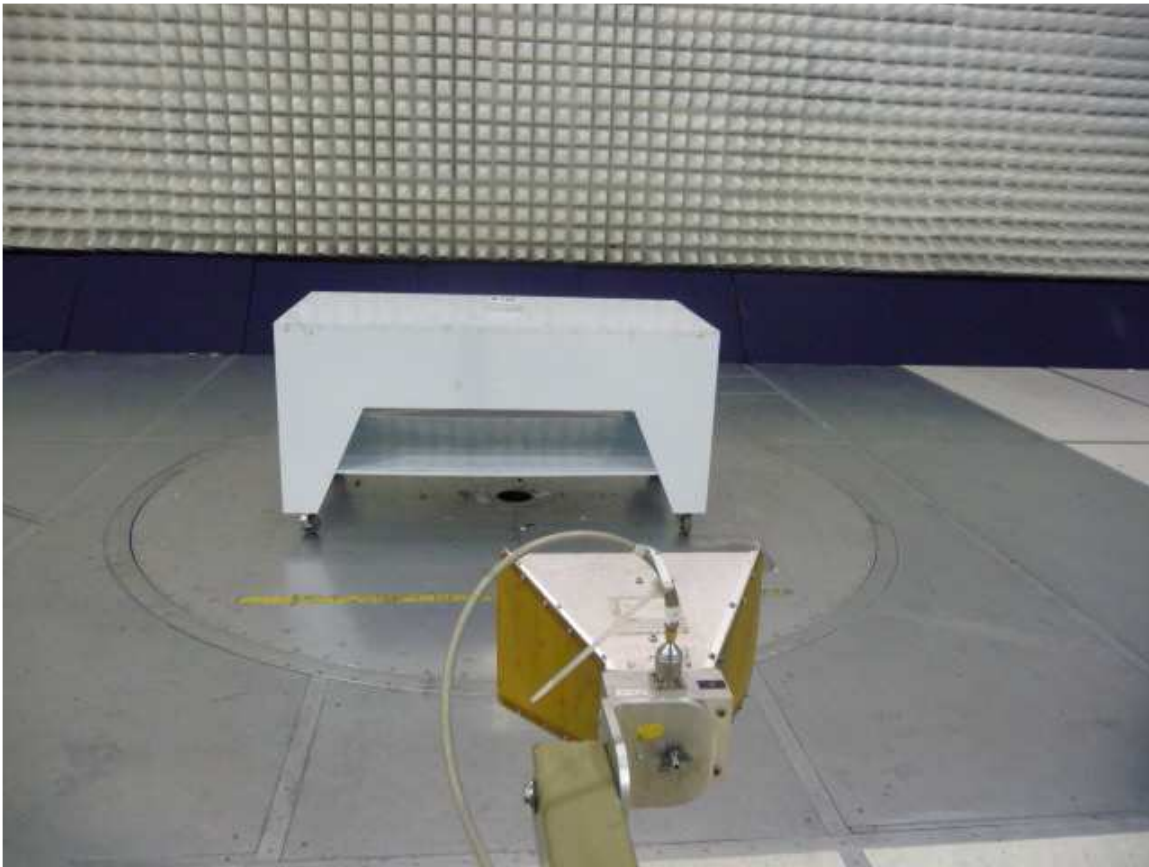
Radiated Emissions at 3 m
