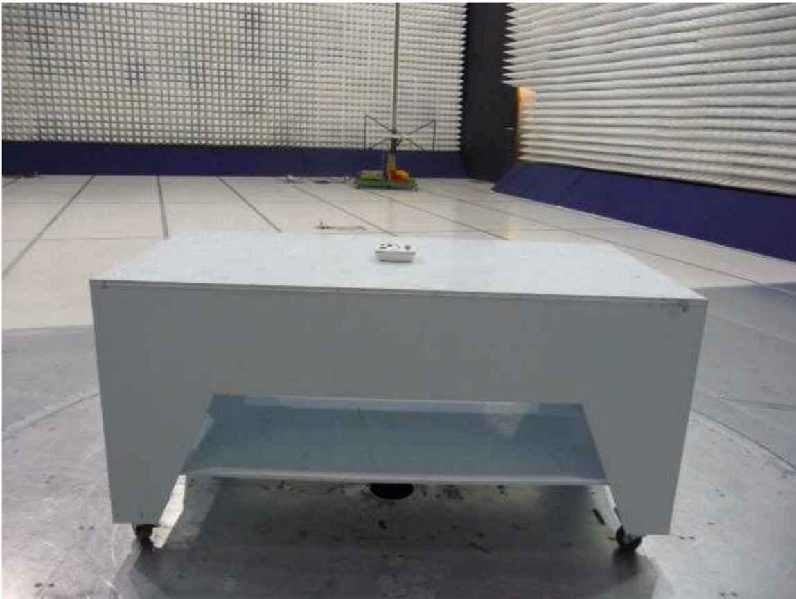
Radiated Emissions at 10 m
