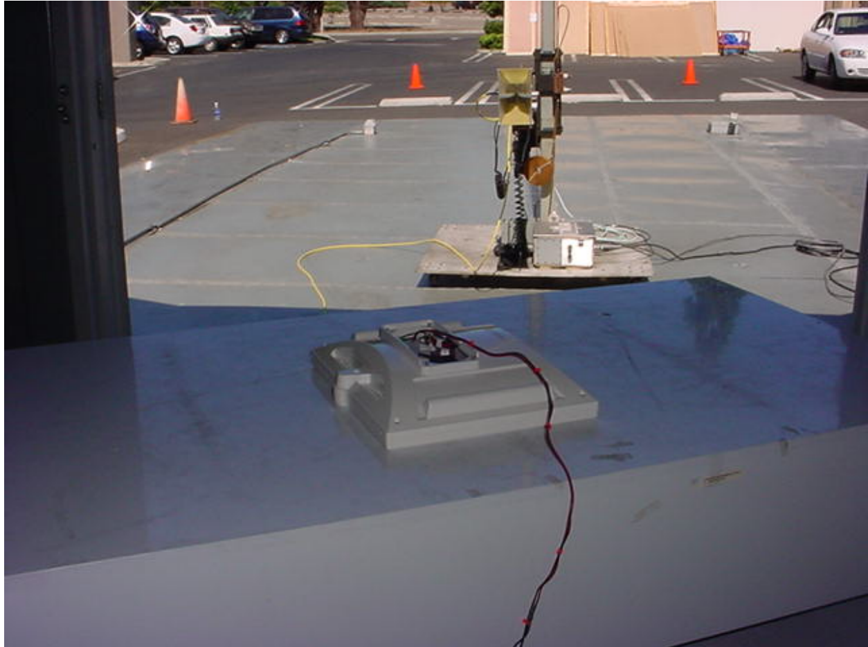
Remote Control Master, Radiated Emission (15.247 / 15.109)
