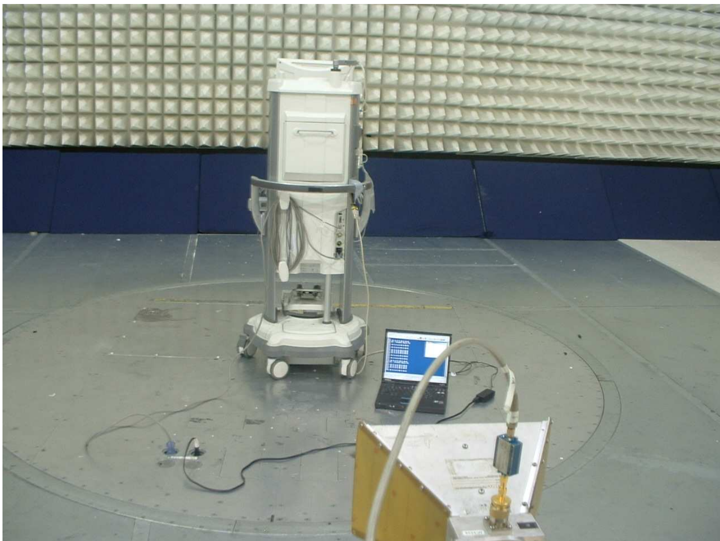
Radiated Emissions at 3 m
