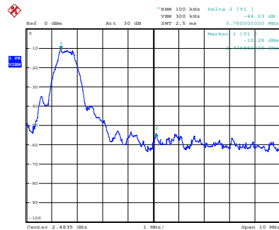
Port 2, 2483.5 MHz Band Edge
