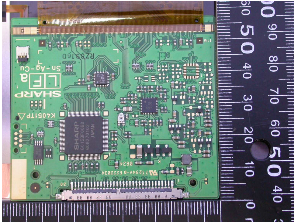
21. Front view of PCB6
