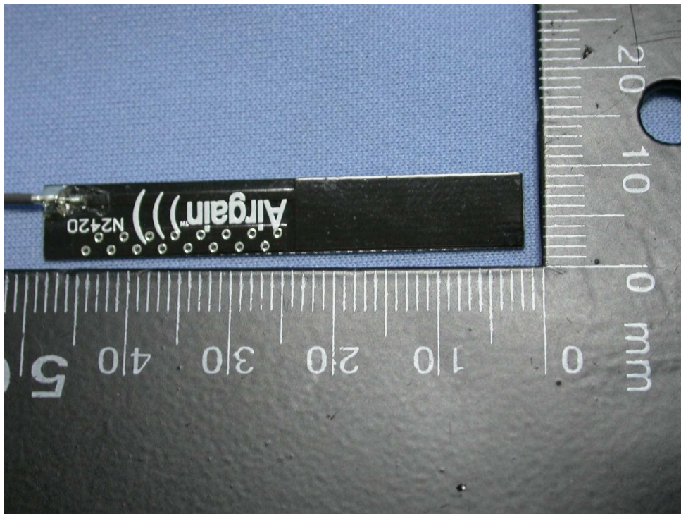
13. Front view of PCB2
