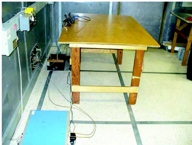
Photographs 1 & 2: Conducted Emission Setup
