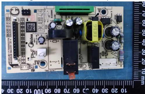
Original Mother board-top view
