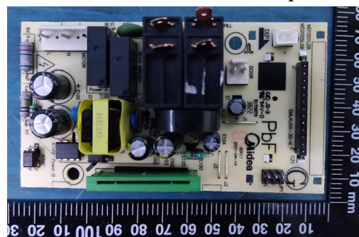
The New Mother board -top view
